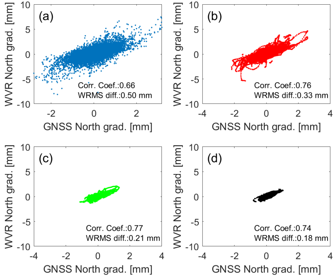
Figure 10. Correlations between estimated north gradients from the GNSS, given by the GRE solution with a 3^\circ elevation cutoff angle , and the WVR data. Four different values of \Delta t_{\text{eff}} (a) 5 min, (b) 2 h, (c) 12 h, and (d) 24 h are used.
