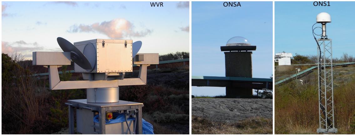
Figure 3. The water vapour radiometer (WVR) Konrad and GNSS sites stations (ONS1 and ONSA) at the Onsala Space Observatory.
