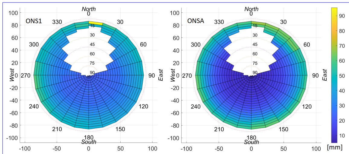
Figure 7. The mean code multipath RMS calculated from ONS1 (left) and ONSA (right).
