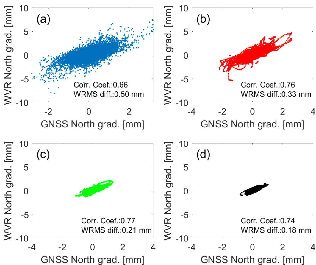
Figure 9. Correlations between estimated north gradients from the GNSS, given by the GRE solution, and the WVR data. Four different values of \Delta t_{\text{eff}} (a) 5 min, (b) 2 h, (c) 12 h, and (d) 24 h are used.
