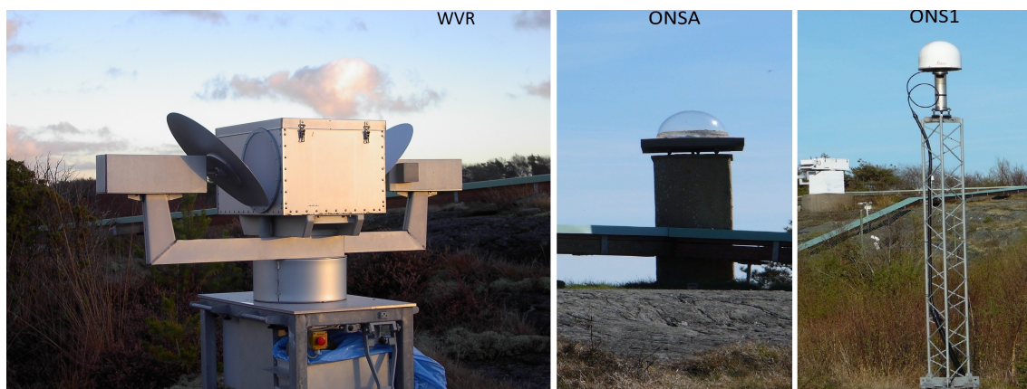
Figure 3. The water vapour radiometer (WVR) Konrad and GNSS sites (ONS1 and ONSA) at the Onsala Space Observatory.
