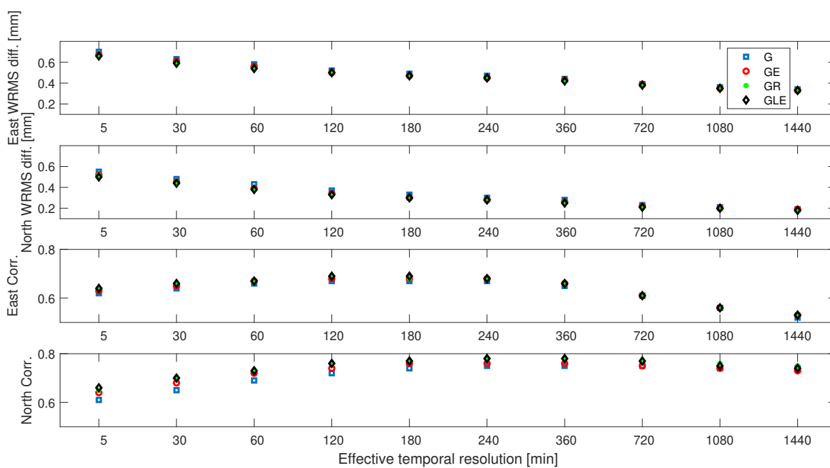
Figure 7. Correlations and WRMS differences between estimated gradients from the GNSS and the WVR data using different effective temporal resolutions, \Delta t_{\text{eff}} .
