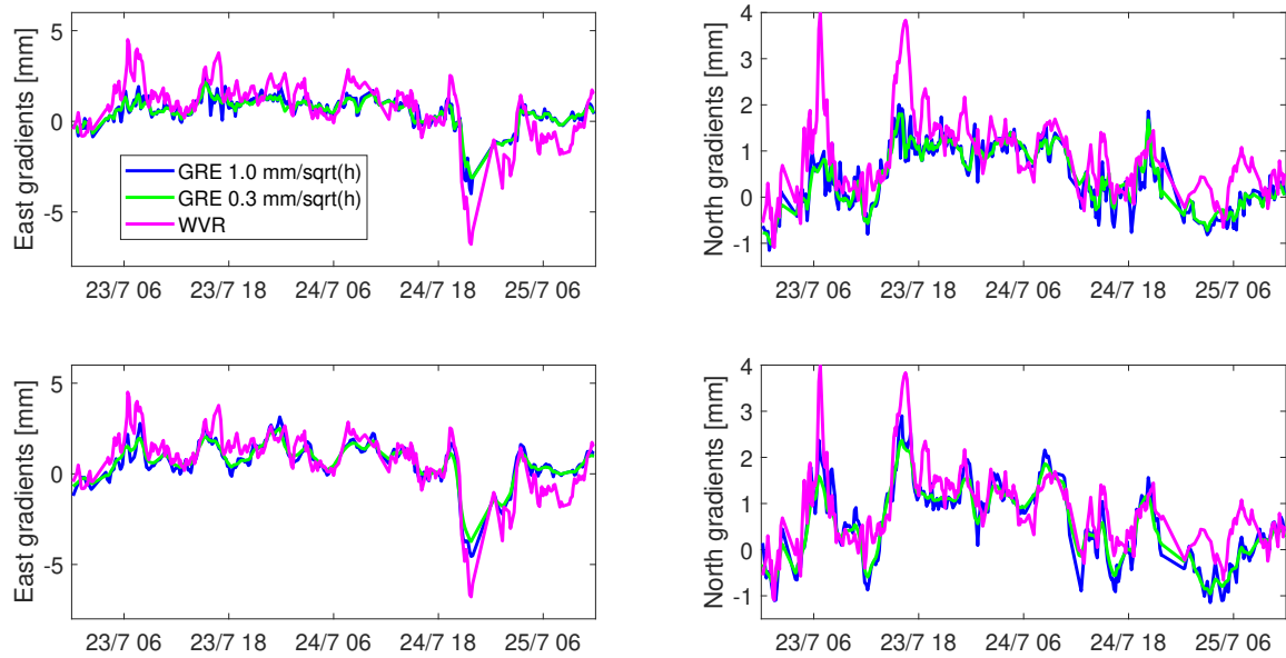
Figure 11. Gradient time series from the WVR and from GNSS (GRE) applying two different constraint values ( 0.3 and 1.0 \text{ mm}\sqrt{\text{h}}^{-1} ) using elevation cutoff angles of 3^\circ (upper panel) and 10^\circ (lower panel).
