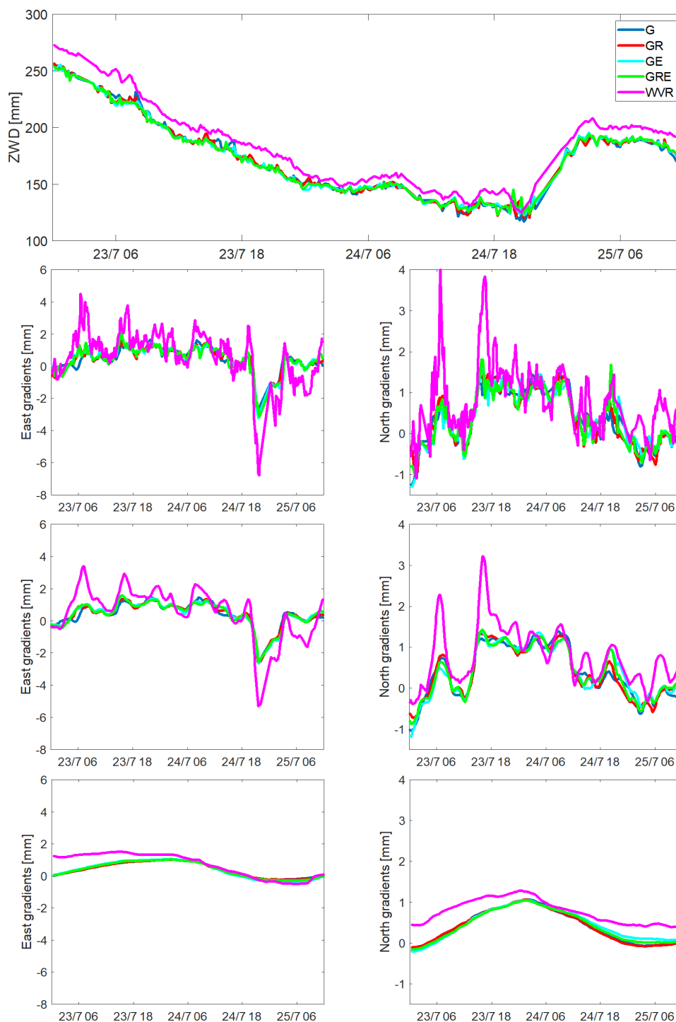
Figure 10. ZWD (top) and gradient time series from the WVR and the GNSS solution using an elevation cutoff angle of 3^\circ . From the second to the bottom panel, east and north gradients are shown for \Delta t_{\text{eff}} of 5 min, 2 h, and 24 h, respectively. Note the different scales for the east and the north gradient graphs.
