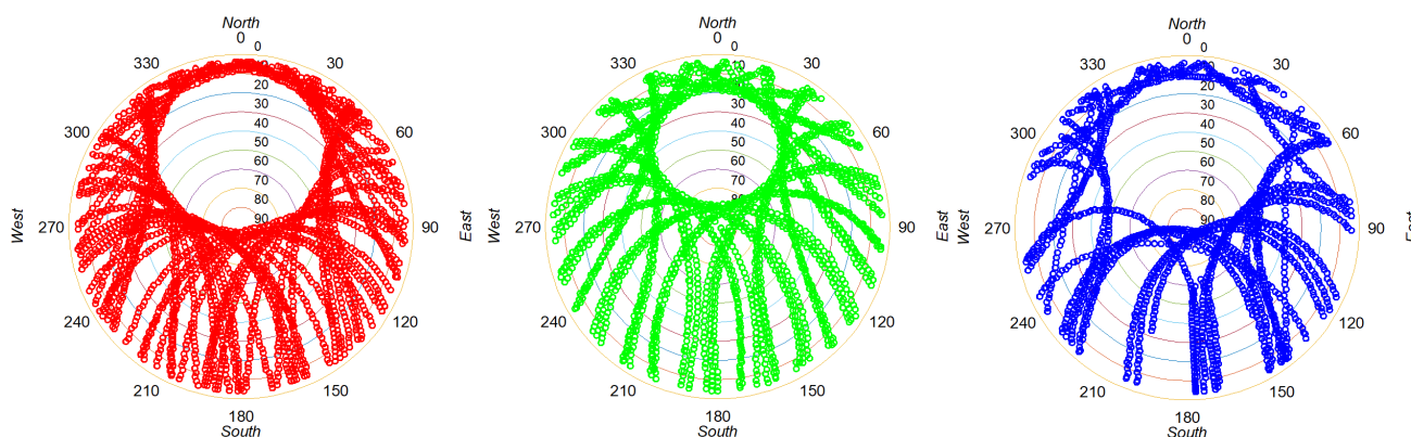
Figure 1. Observations on the sky acquired from ONS1 for 0 to 24 h on July 24, 2019, for GPS (left), Glonass (middle), and Galileo (right).
