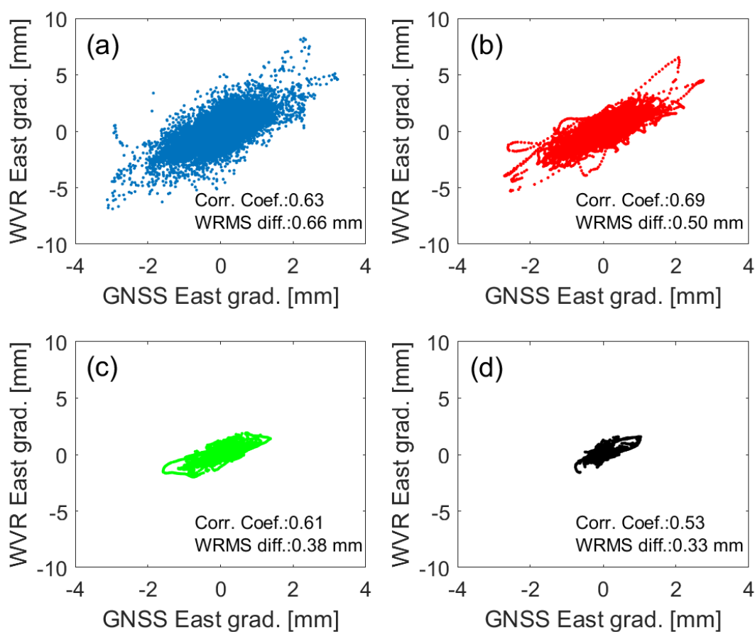
Figure 8. Correlations between estimated east gradients from the GNSS, given by the GRE solution, and the WVR data. Four different values of \Delta t_{\text{eff}} (a) 5 min, (b) 2 h, (c) 12 h, and (d) 24 h are used.
