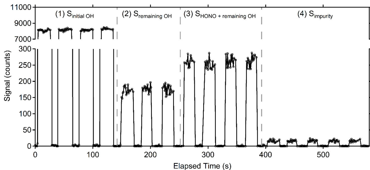
Figure 6: Example of photofragmentation efficiency measurements from an \text{OH} + \text{NO} \rightarrow \text{HONO} calibration. (a) The signal observed from total amount of OH produced in the calibrator ( S_{\text{initial OH}} ). (b) Signal observed from remaining OH after the addition of NO converts the majority of radicals to HONO ( S_{\text{remaining OH}} ). (c) Sum of signal from remaining OH and signal from OH produced in the detection cell after HONO photolysis ( S_{\text{HONO+remaining OH}} ). (d) Signal from the 355-nm photolysis of impurities in the NO cylinder observed when the radical source in the calibrator is turned off ( S_{\text{impurity}} ).
