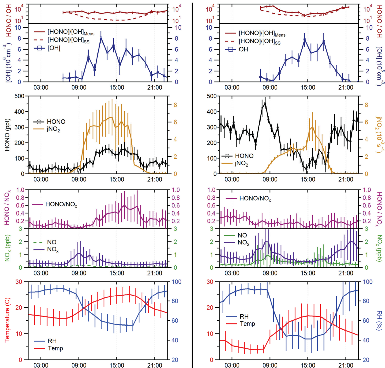
Figure 7: Average measurements of HONO, [OH], HONO/OH, \text{J}(\text{NO}_2) , temperature, RH, \text{NO}_x , and HONO/ \text{NO}_x from the forested site (left) and urban site (right). Mixing ratios of NO at the forested site were estimated based on previous measurements of the \text{NO}/\text{NO}_2 ratio at this site (dashed green line). During the measurement period conducted at the urban site, the detection cell was partially shaded by the building during the morning and early afternoon, resulting in the observed peak in \text{J}(\text{NO}_2) at 15:00. Error bars represent the standard deviation of the diurnal average measurements ( 1\sigma ).
