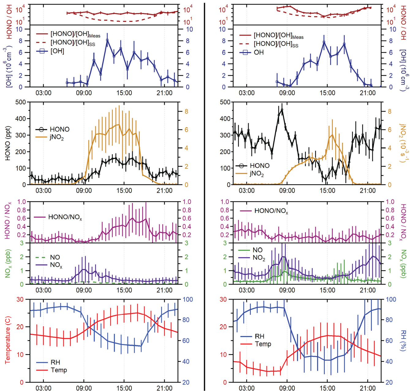
Figure 7: Average measurements of HONO, [OH] , HONO/OH, JNO_2 , temperature, RH, NO_x , and HONO/ NO_x from the forested site (left) and urban site (right). Mixing ratios of NO at the forested site were estimated based on previous measurements of the NO/ NO_2 ratio at this site (dashed green line). During the measurement period conducted at the urban site, the detection cell was partially shaded by the building during the morning and early afternoon, resulting in the observed peak in JNO_2 at 15:00. Error bars represent the standard deviation of the diurnal average measurements ( 1\sigma ).
