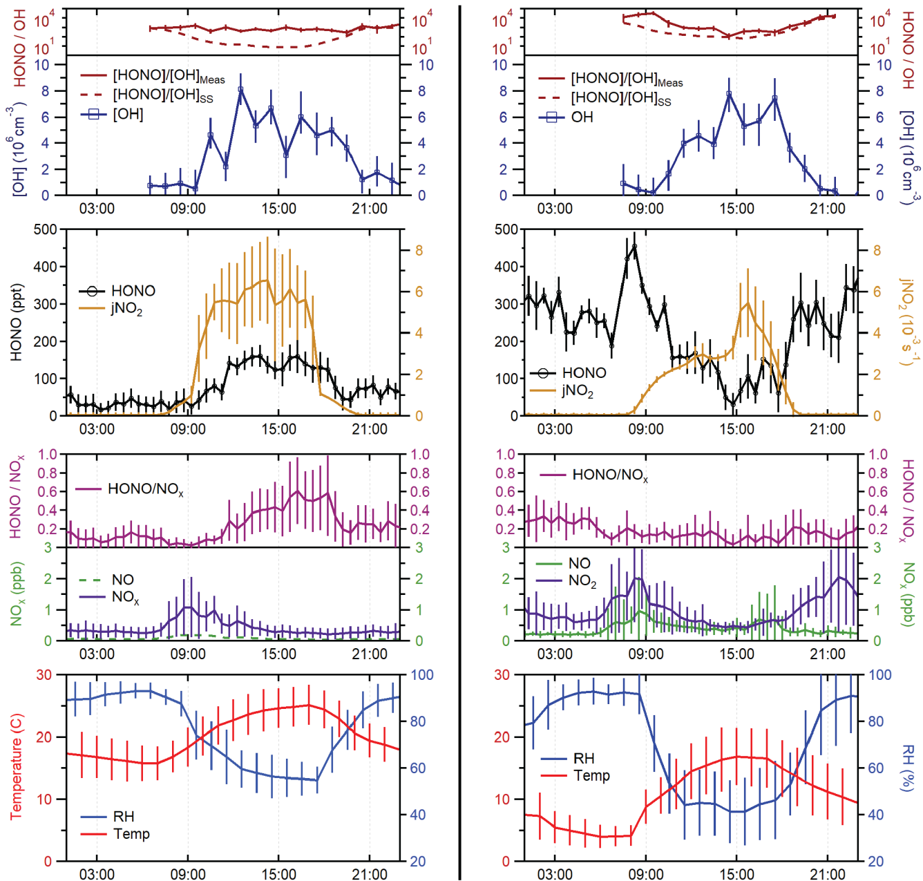
Figure 7: Average measurements of HONO, [OH], HONO/OH, J_{\text{NO}_2} , temperature, RH, \text{NO}_x , and HONO/ \text{NO}_x from the forested site (left) and urban site (right). Mixing ratios of NO at the forested site were estimated based on previous measurements of the NO/ \text{NO}_2 ratio at this site (dashed green line). During the measurement period conducted at the urban site, the detection cell was partially shaded by the building during the morning and early afternoon, resulting in the observed peak in J_{\text{NO}_2} at 15:00. Error bars represent the standard deviation of the diurnal average measurements ( 1\sigma ).
