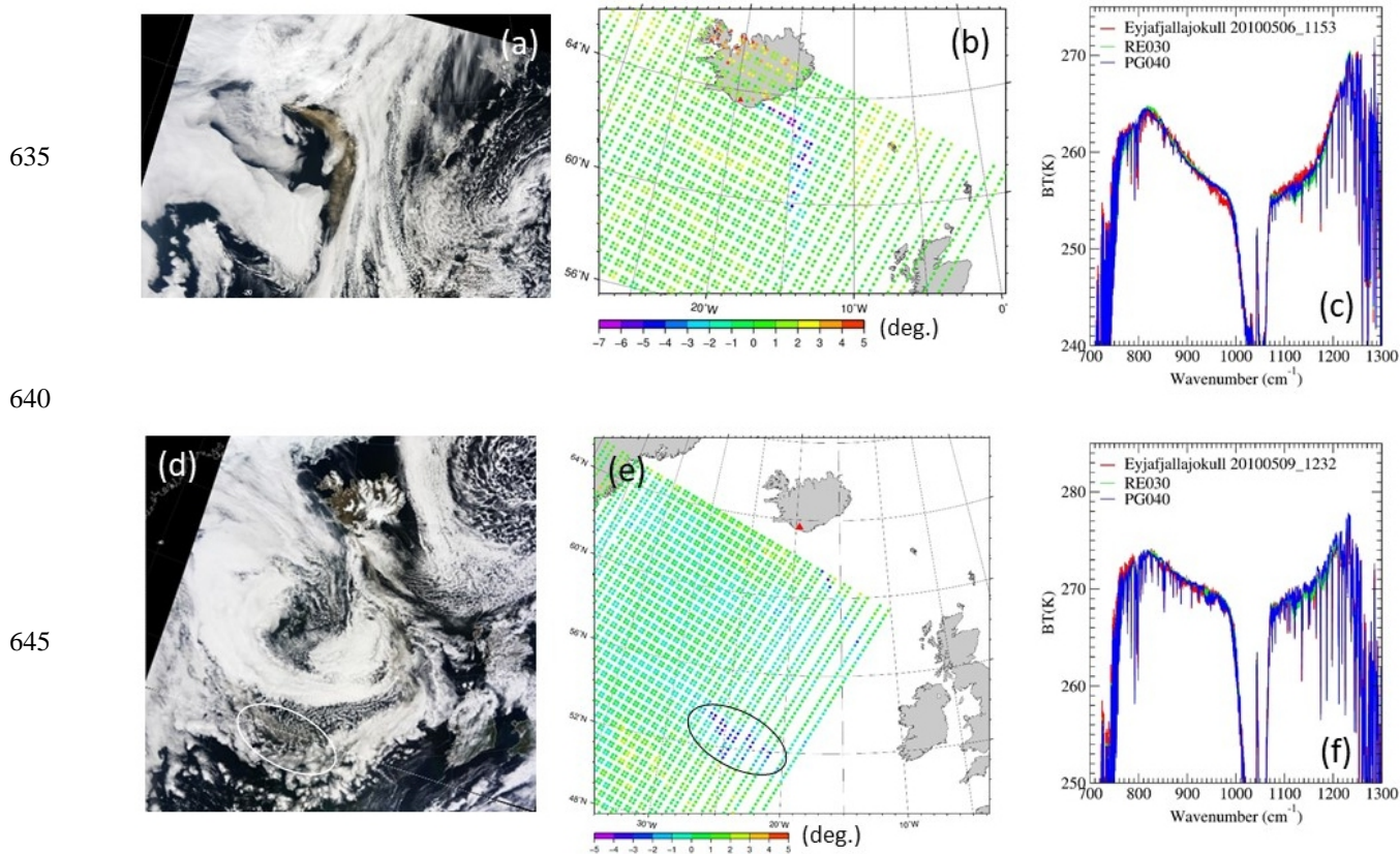
Figure 10: Examples of BTS analyses of the Eyjafjallajökull VAC on 6 May 2010 (a–c). (a) MODIS true-colour image at 11:55 UTC and (b) brightness temperature difference \Delta BT_{split} measured with IASI at 11:53 UTC. (c) BTS of IASI measurement at (lat, lon) = (63.146^\circ N, 15.261^\circ W) (red), and results of BTS simulations using the RI models RE030 (green) and PG040 (blue). (d–f) Same as (a–c), but for the VAC on 9 May 2010. The MODIS colour image is a composite from 12:25–12:30 UTC (d) and IASI \Delta BT_{split} is calculated at 12:32 UTC (e). The area of highly negative \Delta BT_{split} is indicated with circles in (d and e). (f) Measured and simulated BTS for the IASI pixel at (lat, lon) = (52.549^\circ N, 24.075^\circ W) . The retrieved VAC parameters and SO_2 column for each BTS simulation are listed in Table 3.
