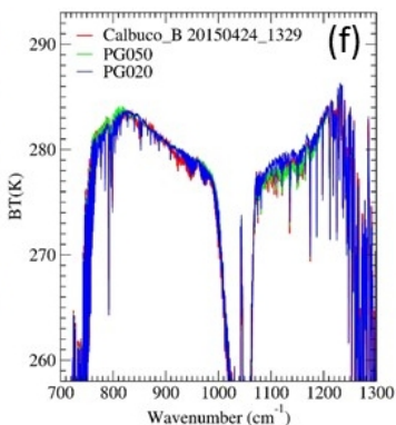
Figure 13: Brightness temperature difference \Delta BT_{split} of Calbuco ash plumes measured by IASI at 13:29 UTC on 24 Apr 2015 over the Atlantic Ocean [Calbuco_A, (b)], and the measured (red) and calculated (PG020, blue) BTS for the pixel at (lat, lon) = (35.336^\circ S, 55.051^\circ W) (c). MODIS visible-colour image of the same region at 13:25 UTC (a). (d–f) Same as (a–c) but for ash plumes over the Pacific Ocean [Calbuco_B, marked with a circle in (e)] and the measured BTS at (lat, lon) = (32.592^\circ S, 75.050^\circ W) . Calculated BTS without SO_2 gas from the PG050 (green line) and PG020 (blue line) RI models are also shown. The measurement time of the MODIS colour image (d) was 15:00 UTC.
