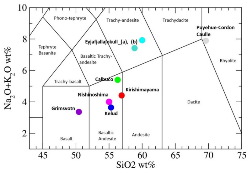
455 Figure 7: Total alkali-silica (TAS) diagram based on ash and pumice samples of the volcanos featured in Table 2. \text{SiO}_2 and \text{Na}_2\text{O} + \text{K}_2\text{O} wt.% values for each volcano were obtained from the literature as follows: Calbuco, Deguine et al. (2020); Eyjafjallajökull and Grímsvötn, Reed et al. (2018) and Prata et al. (2019); Kelud, Maeno et al. (2019); Kirishimayama, https://www.gsj.jp/hazards/volcano/kirishima/2011/works-index.html ; Nishinoshima, https://www.data.jma.go.jp/svd/vois/data/tokyo/STOCK/kaisetsu/CCPVE/shiryo/147/147_2-2.pdf ; Puyehue-Cordón Caulle, Castro et al. (2013).
