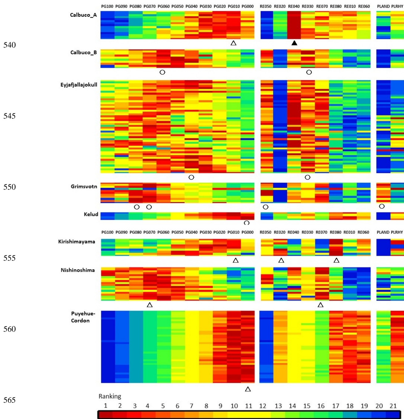
Figure 8: Ranking plots showing the results of BTS simulations for the pixels used for the IASI ash plume measurements in Table 2. The ranking of the 21 RI models is in ascending order of the RMS values between the measured and simulated BTS. Results for
