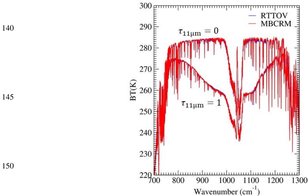
Figure 2: Comparisons of the IASI BTS simulated using MBCRM and RTTOV (ver.12.2) for clear sky ( \tau_{11\mu\text{m}} = 0 ) and cloudy 155 ( \tau_{11\mu\text{m}} = 1 ) atmosphere. Optical depth was defined as that at wavelength 11 \mu\text{m} ( \nu = 907.488 \text{ cm}^{-1} ). The average atmospheric profile in the ECMWF 52 diverse profile dataset (no. 52) and the satellite zenith angle 0^\circ were used, and a sea surface emissivity model and surface temperature 286.52 K were applied. For cloudy atmosphere, a homogeneous aerosol layer between 358.966 hPa and 459.712 hPa, and the aerosol properties of the ‘new volcanic ash (VAPO)’ model in RTTOV (Vidot and Hocking, 2017) were considered. For RTTOV, result of 8 streams discrete-ordinate method (DOM) was plotted. For MBCRM calculations, we read the 160 complex refractive index (RI) data of VAPO from the figure in the RTTOV-11 Science and Validation Report (Saunders et al., 2013).
