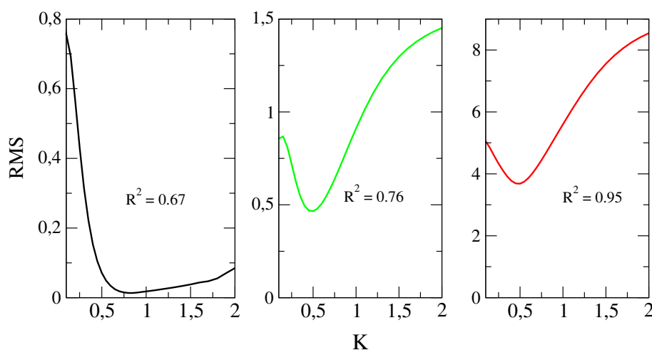
Figure 5. Plots of the curves of the root mean square (RMS) differences between the optical depths retrieved from FIRMOS and the LiDAR as a function of the backscatter extinction coefficient ratio k for the ice (black), mixed (green) and water (red) clouds. R^2 denotes the correlation index.
