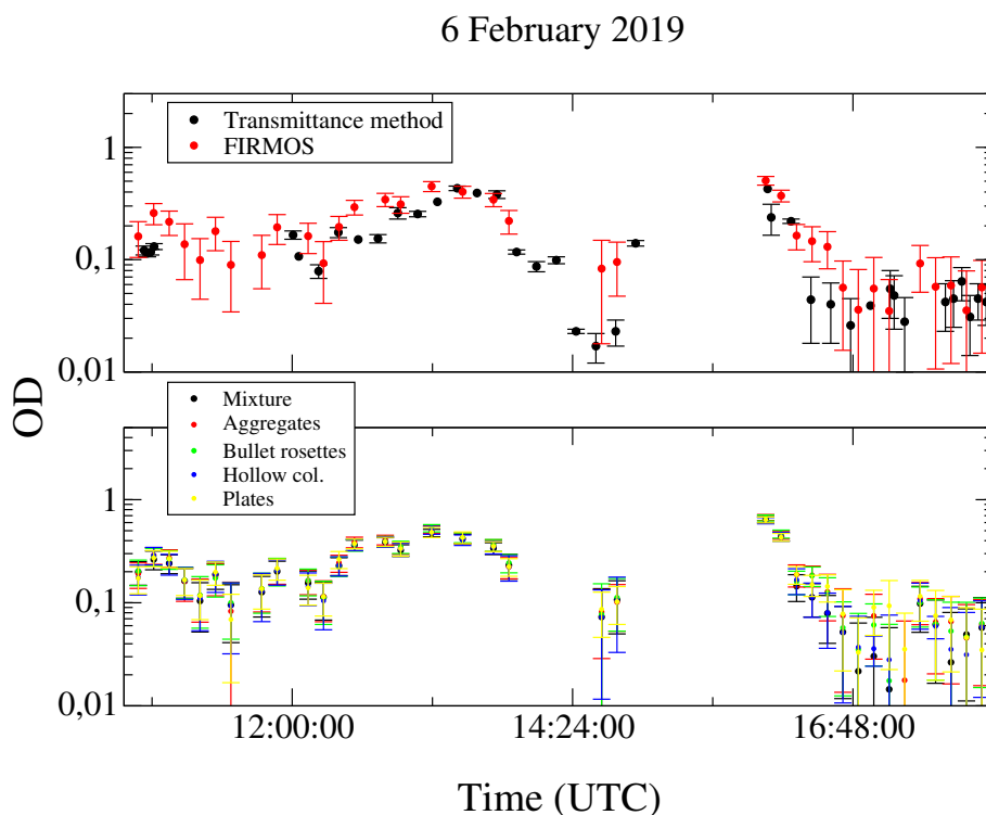
Figure 4. In the upper panel comparison of the ODs retrieved from FIRMOS data (in red) on the day 6 February 2019 and those obtained through the transmittance method (in black). In the lower panel the retrieved ODs from FIRMOS by assuming the mixture (black) and different ice crystals habits (red, green, blue and yellow).
