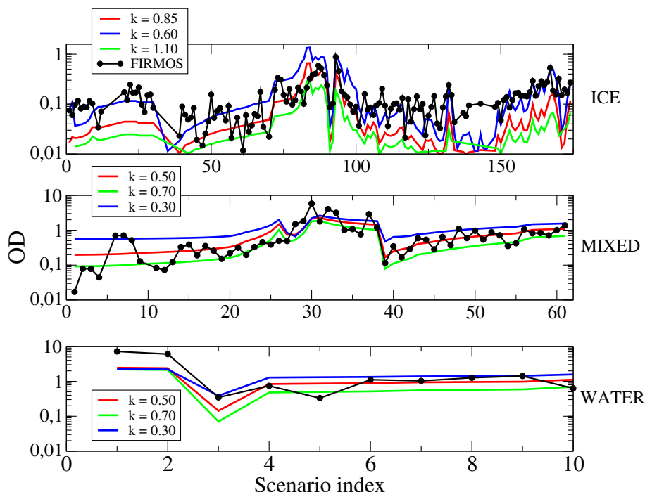
Figure 6. In the upper, middle and lower panel the comparison of ice, mixed and water cloud ODs retrieved from FIRMOS (black dots) with those obtained with the Klett approach from LiDAR measurements. The red lines indicate the retrieved OD by using the k of the best fit, while the green and the blue lines show the variability.
