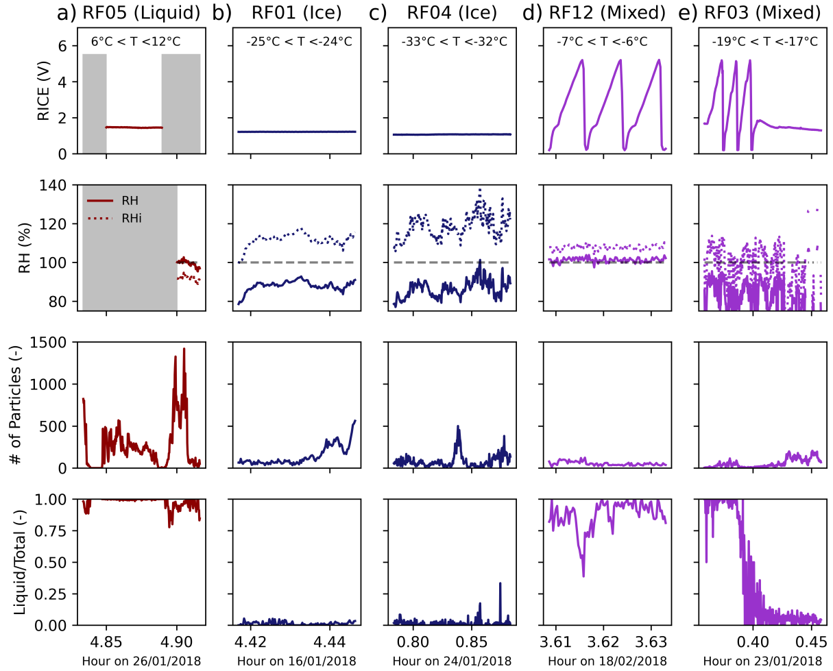
Figure 4. Time series of atmospheric parameters and particle properties for the liquid-only period (a) and the two ice-dominated periods (b,c), and the two example mixed-phase periods (d,e). Voltage from the RICE (row 1), relative humidity with respect to liquid (solid line) and ice (dashed line) (row 2), the number of particles that satisfy our selection criteria (row 3), and liquid fraction as determined by the UWILD algorithm (row 4) are shown for each flight period. A RICE response is expected when the supercooled liquid-water content exceeds 0.01 \text{g m}^{-3} . Missing data are indicated with grey. The temperature range sampled in each period is shown on the plot of RICE voltage in the top row.
