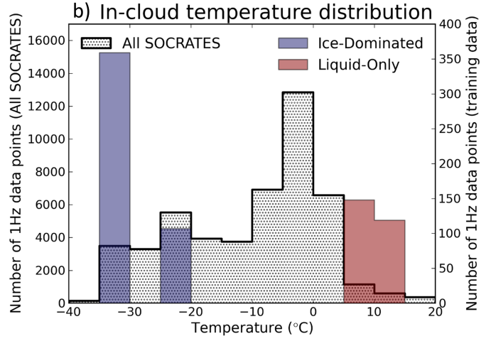
Figure 2. A-(a) SOCRATES flight tracks from RF01-RF14 (the flights analyzed in this study). B-(b) 1-Hz in-cloud temperature histograms for RF01-RF14 (hatched, left y-axis), ice-dominated data from the TTV set (blue, right y-axis) and liquid-only data from the TTV set (red, right y-axis). In-cloud data includes all samples with at least 1 particle that satisfy our selection criteria (described in Section 22.1).
