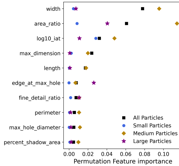
Figure 6. Permutation feature importance for the ten most important features is shown for all particles (black squares) and for the three size classes separately . Features are shuffled ten times and the mean feature importance from the ten trials is shown here.
