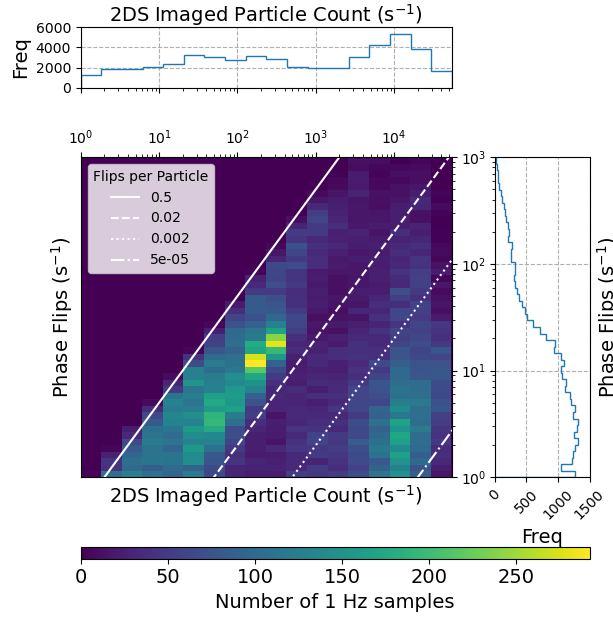
Figure 11. A 2D histogram of 1-Hz particle phase flips (y-axis) and 1-Hz 2D-S-imaged-total particles (including both successfully classified particles and unclassifiable particles) is shown in the top-row large plot . A 1D histogram of 1-Hz 2D-S-imaged-totsl particles is shown on top, on a shared x-axis, and a 1D histogram of 1-Hz phase flips per second is shown on the right, on a shared y-axis. A value closer to the upper left of the plot indicates a higher degree of particle heterogeneity. White lines indicate lines of constant heterogeneity for varying particle counts. Data are from all SOCRATES flights RF01-RF14 are included .
