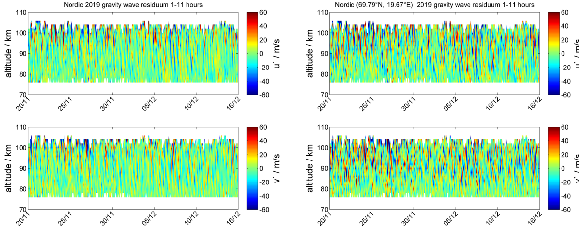
Figure 11. The left two panels show the zonal and meridional gravity wave residuum for all waves in the period range between 1 to 11 hours with color-coded amplitude integrated over the Nordic domain from 20th of November 2019 to 15th of December 2019. The right two panels highlight the same but for the grid cell located around geographic latitude ( 69.79^\circ N, 19.67^\circ E) down to horizontal scales of 60 km.
