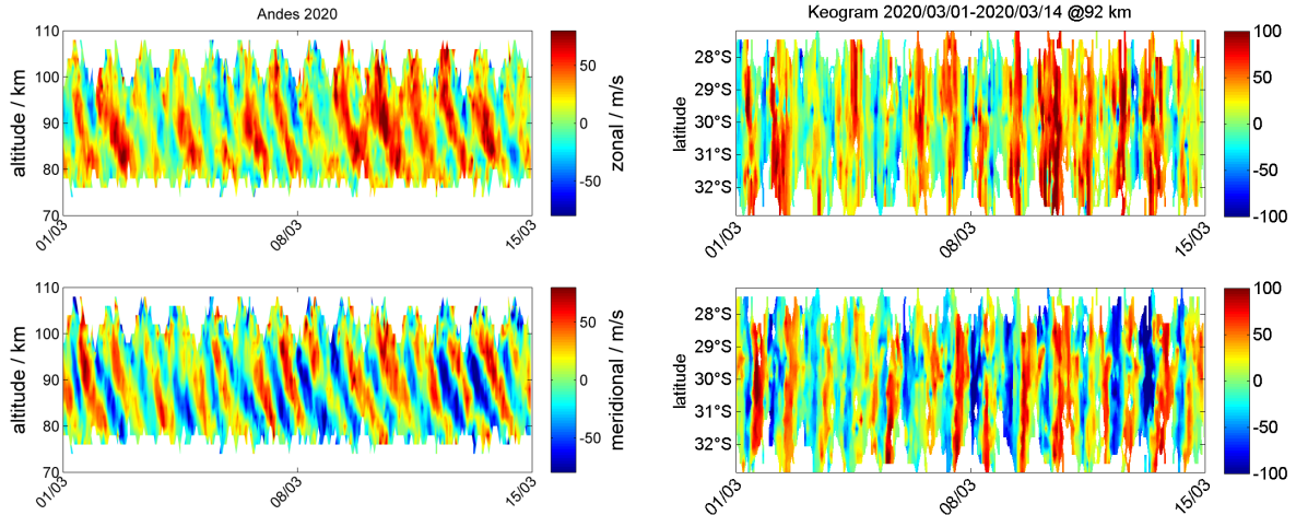
Figure 13. The two panels show a ATW measured with CONDOR and the corresponding Keogram for the altitude of 92 km. The data was recorded between 1st to 14th March 2020.
