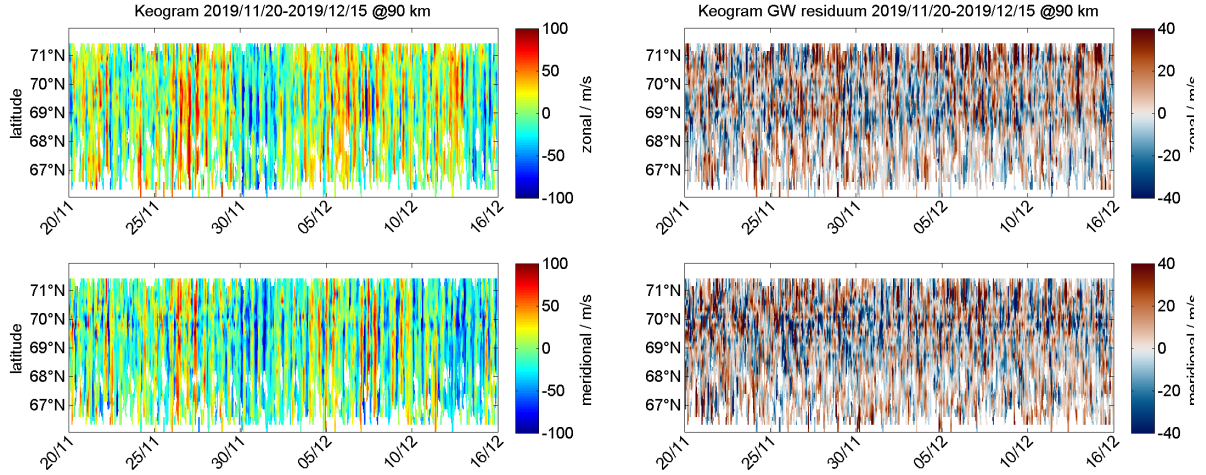
Figure 12. The two panels show color-coded latitudinal keograms of zonal and meridional winds for 22° longitude and 90 km altitude from 20th November 2019 to 15th December 2019.
