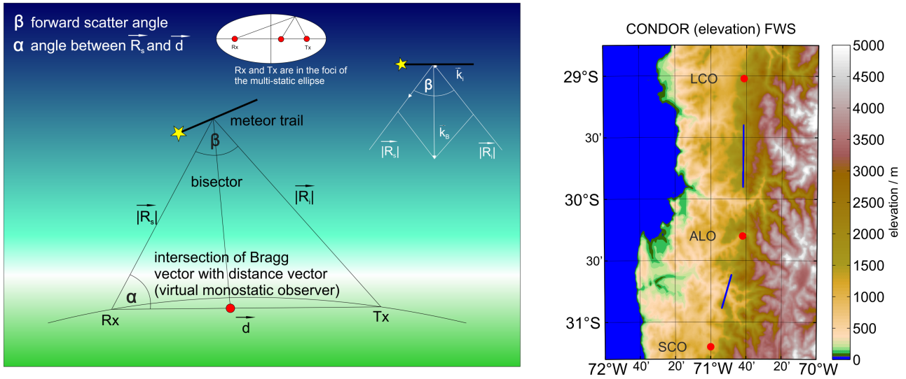
Figure 3. Left panel: Schematic representation of the forward scatter geometry and Bragg vector for CONDOR. Right panel: Geographic map of CONDOR with the active and passive radar locations at ALO, SCO and LCO (red dots). The two set of intersection points of the Bragg vectors with the distance vector between Rx and Tx are shown as blue dots, which are only visible as two blue streaks due to the close proximity of the intersection points.
