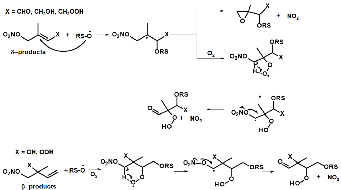
Figure 9: Possible mechanism for surface-catalysed conversion of first generation ISOP-NIT in TDI-1. RS-O represents a reactive surface site.
