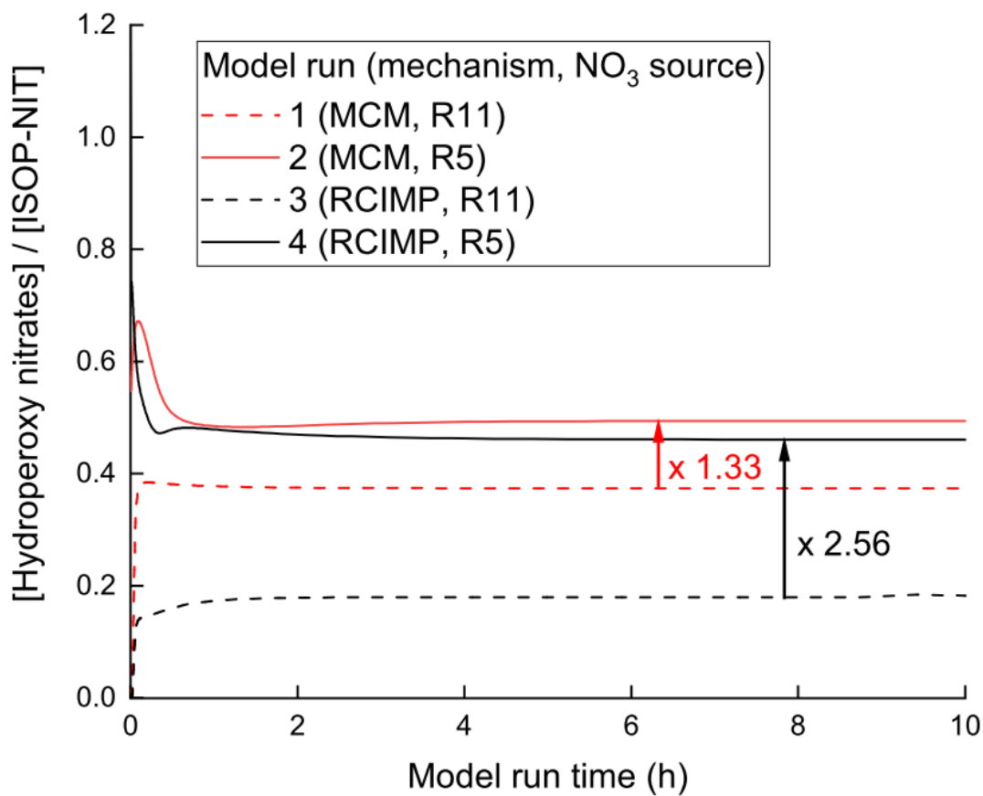
855 Figure 10: Simulated fractional contribution of hydroperoxy nitrates to ISOP-NIT using schemes taken from the MCM (red) and from RCIMP (black). The simulations reproduce the experimental conditions in Fig.3 and Fig.6, with 22 ppbv of isoprene together with either 3 ppbv N 2 O 5 as NO 3 source (runs 1 and 3) or 10.8 ppbv NO 2 + 150 ppbv O 3 (runs 2 and 4).
