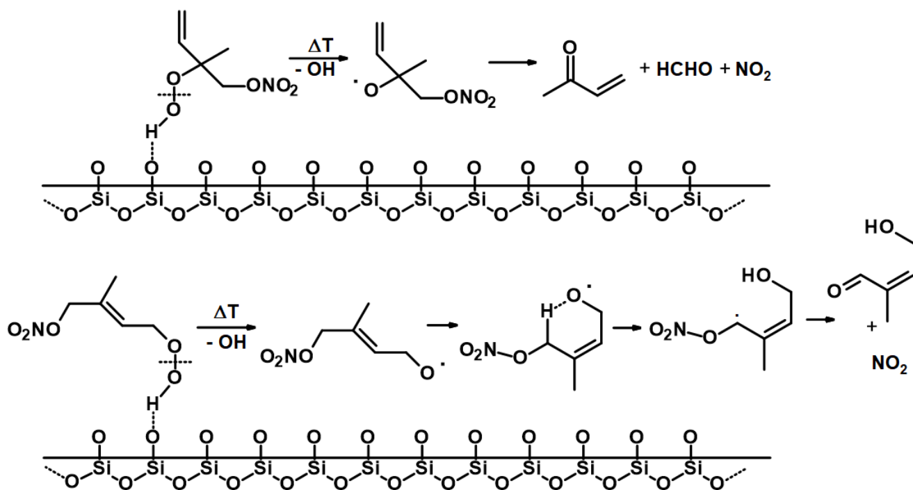
865 Figure 11: Potential degradation pathways of isoprene-derived hydroperoxides on a heated quartz surface.
