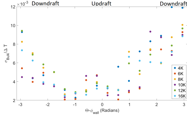
Figure 10. \sigma_T normalized by \Delta T as a function of the angular distance-displacement from the updraft. The temperature was filtered using a high pass Fourier filter with the cutoff at around 5 min.
