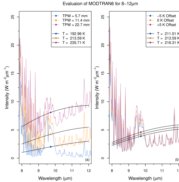
Figure A2. (Left) Downward radiances at the surface, between 8 and 12 \mu m, computed using MODTRAN6 with a midlatitude summer model atmosphere. Water vapor was uniformly scaled to produce a PWV of 5.7 mm (blue), 11.4 mm (orange), and 22.7 mm (purple), with all other model parameters held constant. Also plotted are blackbody curves for three different temperatures (black), with each curve having the same integrated radiance as the corresponding MODTRAN6 radiance. (Right) Same as Left but for uniform changes in atmospheric temperature of \pm 5 K with water vapor held constant at PWV=11.4 mm. Equivalent blackbody curves and temperatures are also shown.
