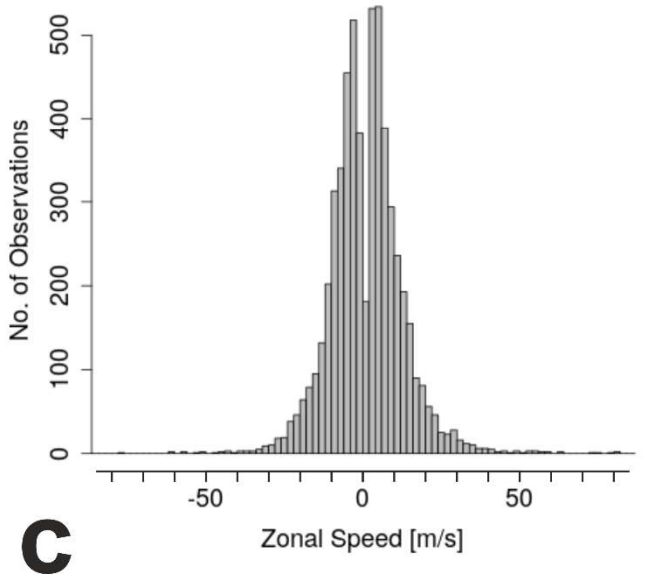
530 Figure 2. Statistical distribution of observed parameters for wave events with horizontal wavelengths between 48 m and 4.5 km from 26 October 2017 to 6 June 2019 at Otlica, Slovenia. a) Period. b) Absolute horizontal phase speed. c) Zonal phase speed. d) Meridional phase speed.
