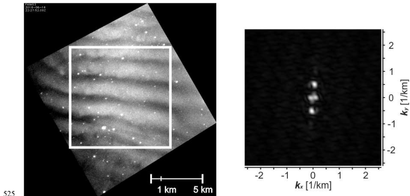
Figure 1. Event from 16 June 2018 22:27:52 UTC. The structure has a horizontal ‘wavelength’ of ca. 1.9 km and extends over the entire image (left). The white square marks the area which is analysed with the 2d-FFT. The respective 2-dimensional spectrum is shown on the right-hand side in the k-space.
