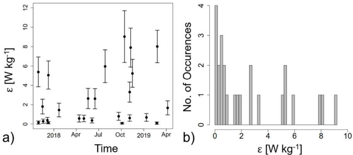
545 Figure 5. a) Temporal evolution of energy dissipation rate of observed turbulence events at OTL (see Table 1). b) Histogram of \epsilon .
