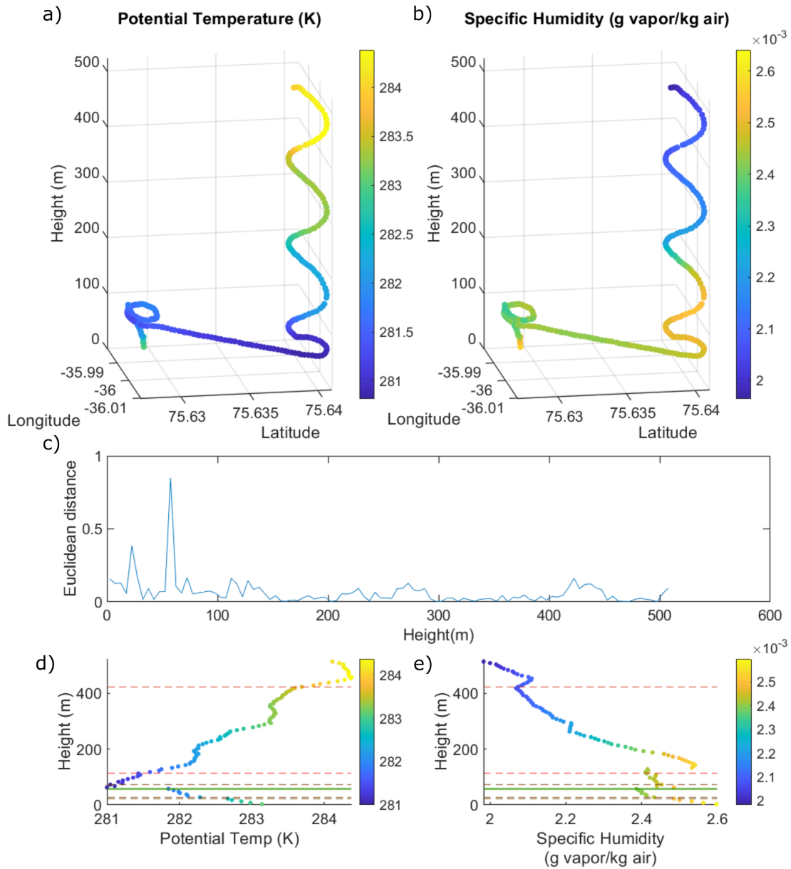
Figure 9: The ascension profile for the June 21st flight mission available to the operator to determine PBL location. The flight reached a maximum altitude of \sim 500\text{m} (a and b). Post launch, the operator flew from the initial launch at \sim 110\text{m} AGL to \sim 60\text{m} AGL over the course of \sim 1 minute. Settling of both temperature and humidity due to hysteresis during that time was flagged incorrectly by Euclidean distance (c). The resulting predictions of PBL locations (solid green line for the most likely, dashed line for the next four likely, d-e) are scattered across the space.
