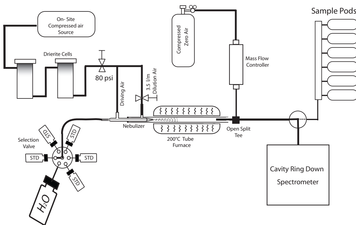
Inlet system to introduce water standard and samples to CRDS System
