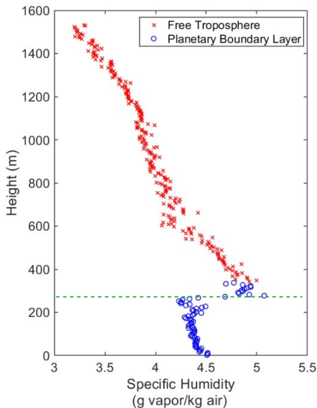
340 Figure 6: The Calinski-Harabasz criterion index (CHCI) applied to the sampling flight on June 12th with a-priori assumption of K=2 . Groups are assumed to represent the free troposphere and PBL, though more structure may exist. The boundary at ~325 m using CHCI is not in agreement with that determined using the Euclidian distance in Figure 7, which shows a likely boundary at ~275 m. This value was chosen by the operator of the flight and shown as the dashed green line. Figure 10 shows an example of a failure in Euclidian distance to predict the boundary layer. The use of CHCI improves the PBL prediction algorithm, as 345 determined in this study.
