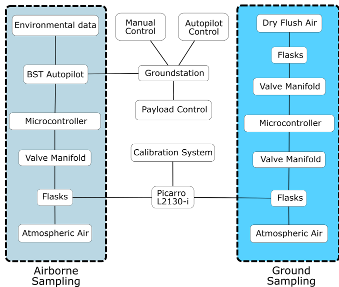
505 Figure A1: UAV-isotope system diagram showing control and sample exchange between airborne/ground sampling and measurement subsystems. Both ground and airborne sampling are performed identically though their control methods differ.
