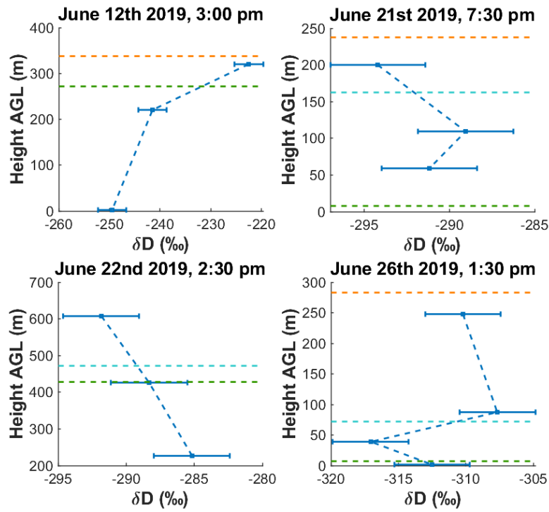
525 Figure A7: A comparison between different methods of determining the location of the PBL. The location predicted from the first off-diagonal of Euclidean distance is indicated by the green dashed line. When the CHCI prediction is different, it is plotted in
