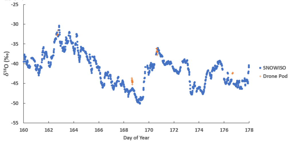
515 Figure A4: Comparison in \delta^{18}O between the tower setup present at the EastGRIP camp in 2019 and 2 meter pod intercomparison measurements. Drone pod measurements on 163 DOY (Day of Year) and 176 DOY correspond to flask measurements taken at 2 meters during a flight mission. All measurements from both tower and UAV are tied to the same isotopic water standards listed in Table 1.
