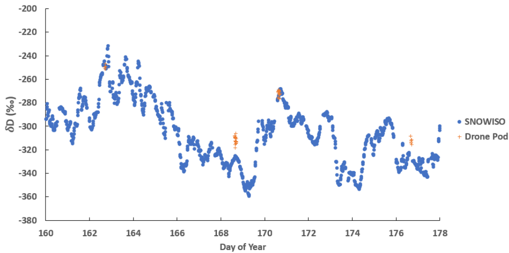
510 Figure A3: Comparison in \delta D between the tower setup present at the EastGRIP camp in 2019 and 2 meter pod intercomparison measurements. Drone pod measurements on 163 DOY (Day of Year) and 176 DOY correspond to flask measurements taken at 2 meters during a flight mission. All measurements from both tower and UAV are tied to the same isotopic water standards listed in Table 1.
