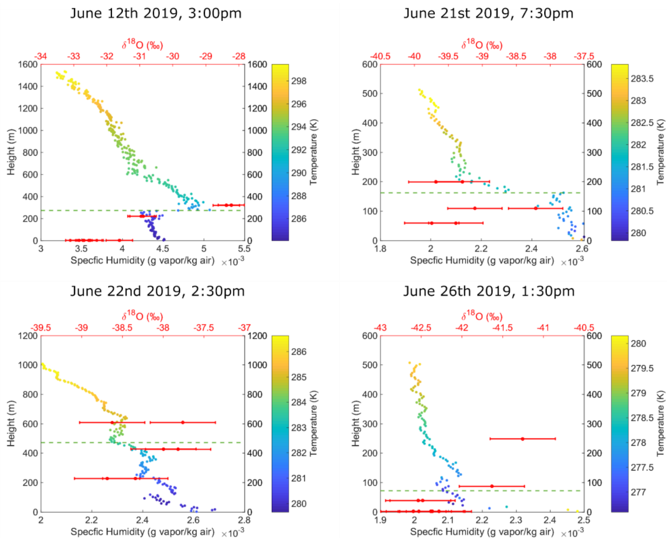
520 Figure A5: The four flights during the 2019 summer field session at EastGRIP field camp. Includes collected environmental data during flight for both ascent and descent as well as measured isotope values for oxygen.
