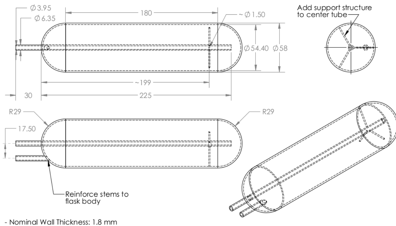
Figure A2: Design document for the glass flasks onboard the S2 payload.
