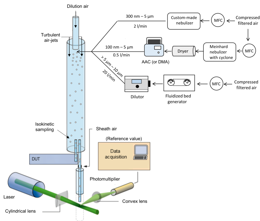
Figure 1. Schematic illustration (simplified) of the primary standard at METAS. MFC, DMA and AAC stand for mass flow controller, differential mobility analyser and aerodynamic aerosol classifier, respectively. For a more detailed description of the experimental setup and the isokinetic sampling probes, readers are referred to Horender et al. (2019) and Vasilatou et al. (2021).
