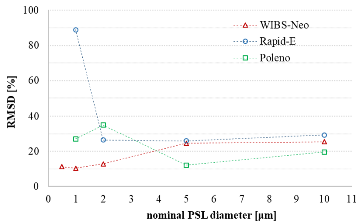
Figure 3. Root mean square deviation between normalized DUT and reference measurements. The value for 2 \mu\text{m} is the mean value of the three measurement sequences with similar diameter (2.07 \mu\text{m} , 2 \mu\text{m} , and 2.1 \mu\text{m} ).
