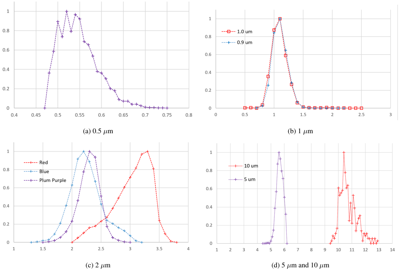
Figure 4. Size distribution estimated by the WIBS-NEO for different PSL particles with diameters ranging from 0.5-10 \mu\text{m}
