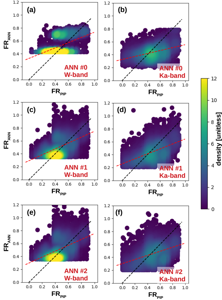
Figure 2. scatter Scatter plots of ANN performances on the test set. The black dashed line marks the 1:1 line, the red dashed line is a linear model fit to the data. The slopes of the red dashed lines are listed in Table 2. (a) W-band, ANN #0; (b) Ka-band, ANN #0 (c) W-band, ANN #1; (d) Ka-band, ANN #1; (e) W-band, ANN #2; (e) Ka-band, ANN #2
