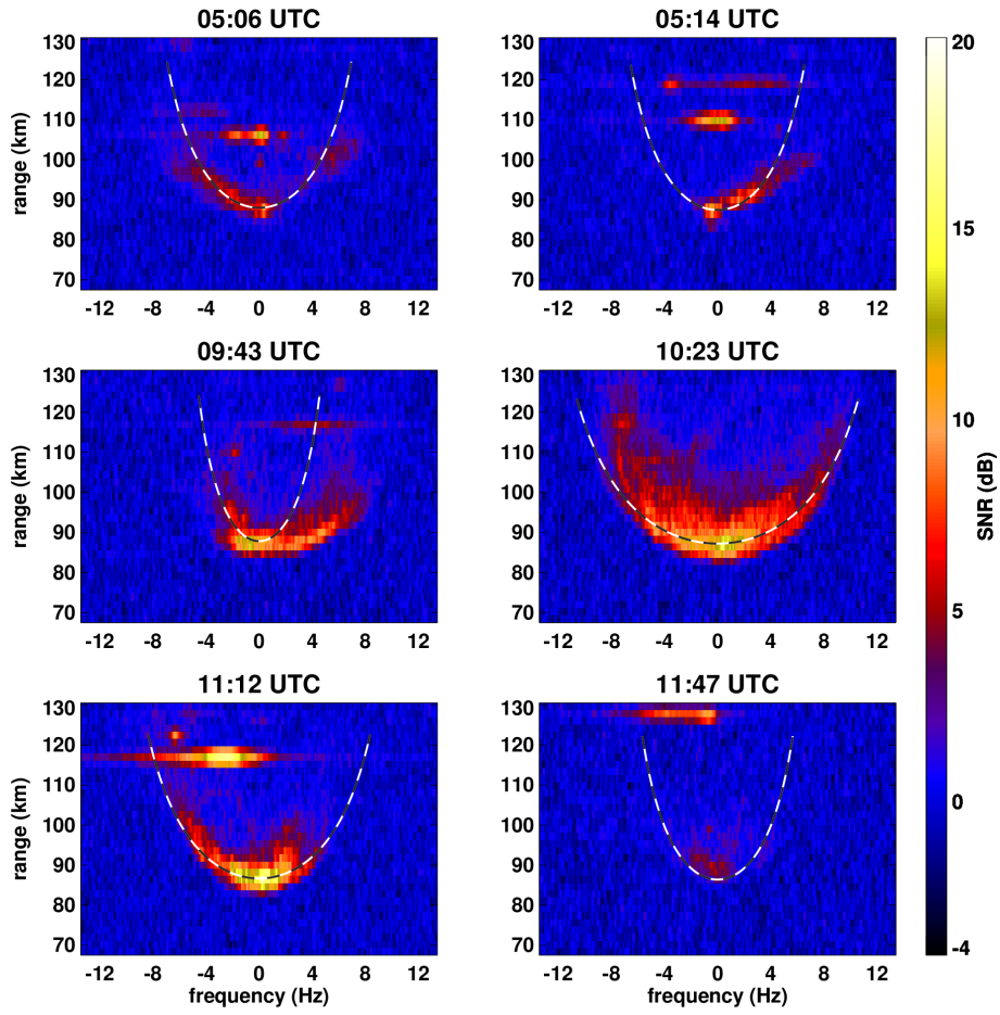
Figure 4. NMSR range-Doppler profiles for 19 July, 2020 ( 0.018 Hz frequency resolution ), constructed from one minute observation periods. Top left: transient PMSE detection. Top right: Asymmetric transient PMSE. Middle left: Asymmetric onset of strong PMSE return. Middle right: strong PMSE return exhibiting fine structure. Bottom left: end of strong PMSE period displaying asymmetric intensity distribution. Bottom right: End of PMSE detection period primarily around 0-Doppler. Dashed lines show the expected range-Doppler profile of a thin layer, based on speed calculated from meteor trail detection radial velocities.
