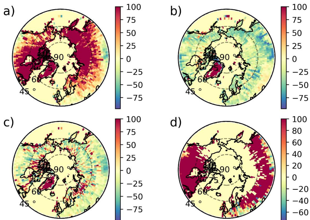
610 Figure 8 Polar plots of the percent difference in the number of soundings that pass the NN filter compared to the qc_flag filter for spring (a), summer (b), fall (c), and winter (d). The data have been binned by 2° longitude by 2° latitude.
