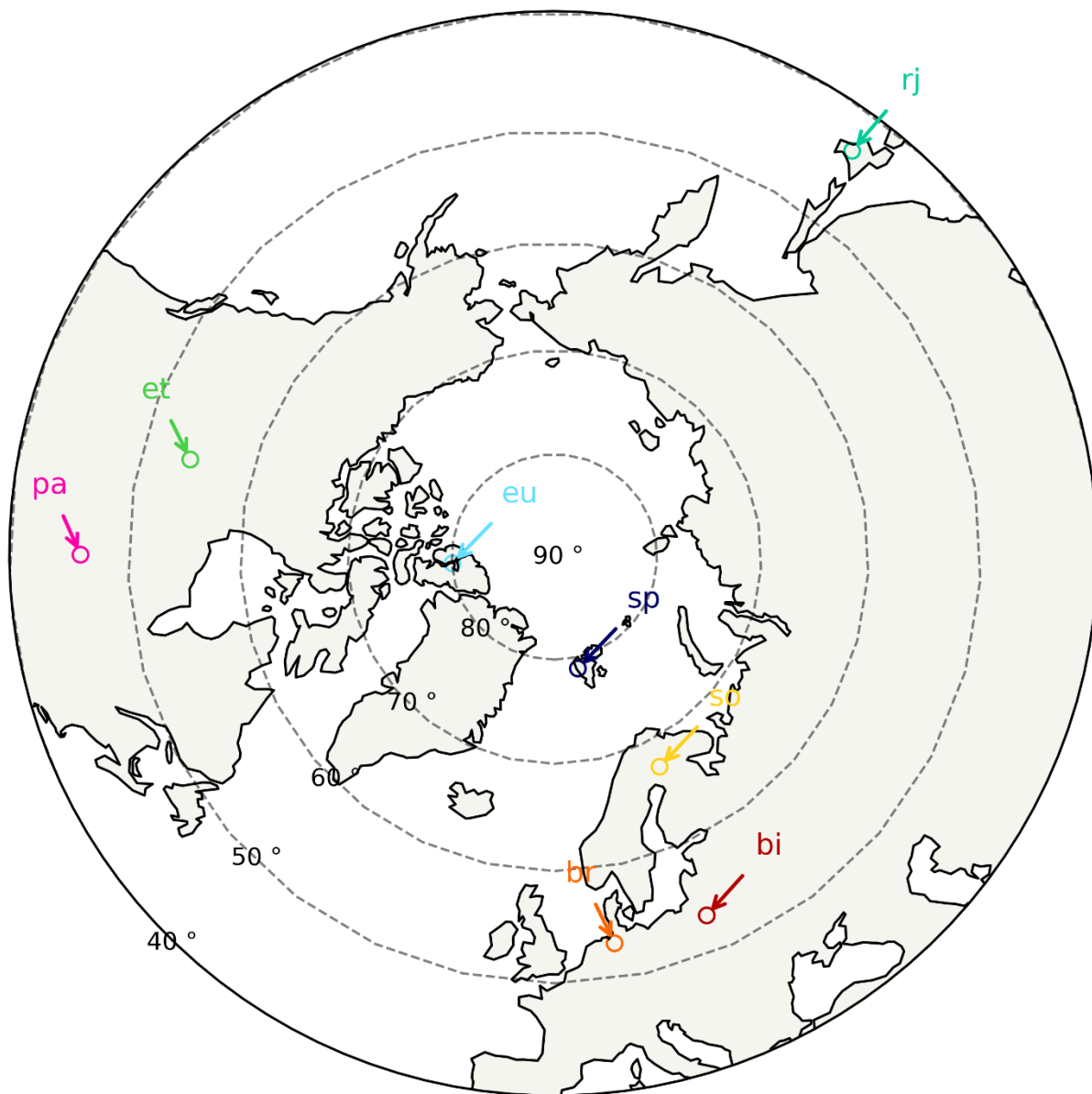
580 Figure 1: Map of the location of all TCCON sites used in this study.
