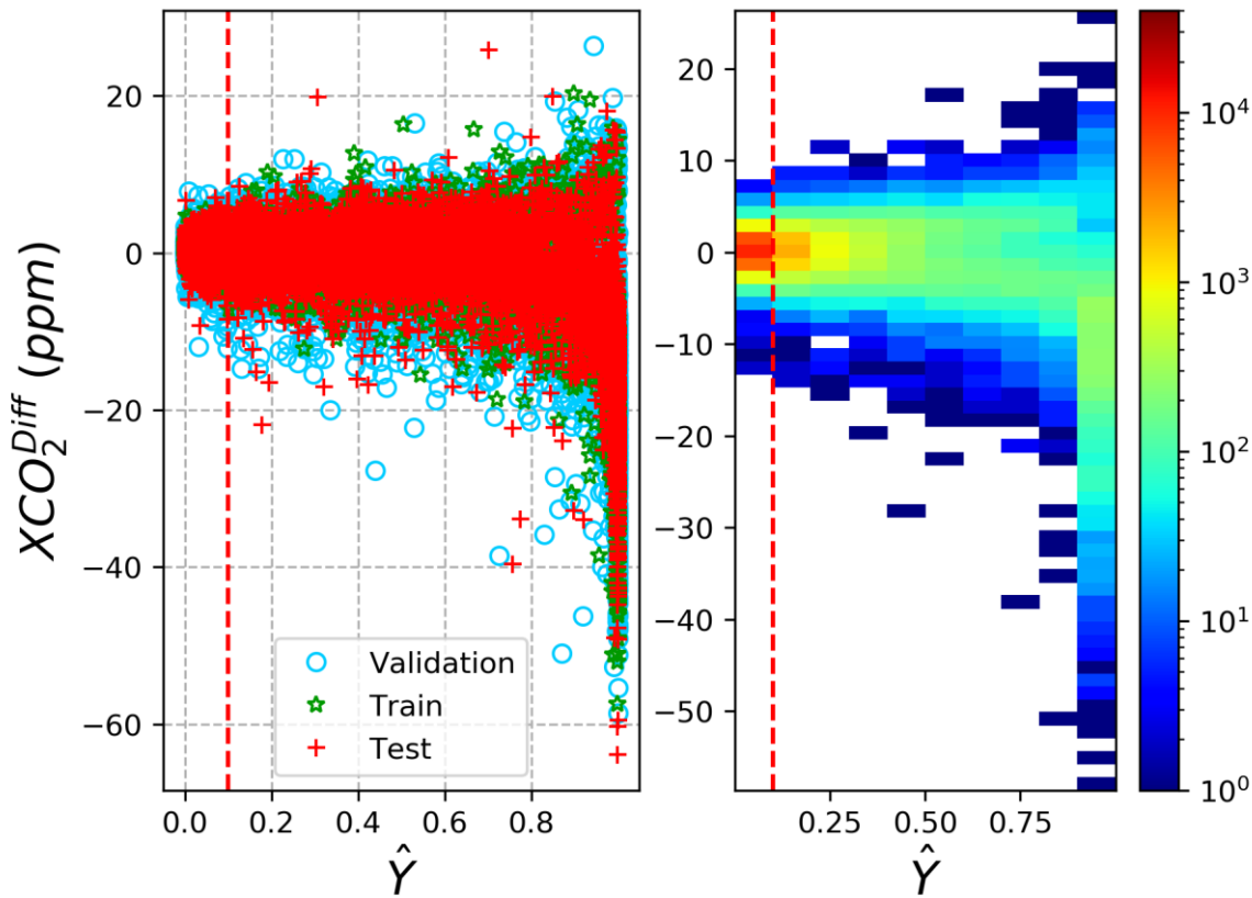
585 Figure 3 a) The difference between the coincident TCCON and OCO-2 retrievals ( XCO_2^{Diff} ) as a function of \hat{Y} calculated by the NN (after training) for the training, testing, and validation data sets. b) Same as plot a) but shows the density of the all three data sets combined, with the color bar given on a log scale. The red dashed lines represent the boundary between setting the binary classification of the data.
