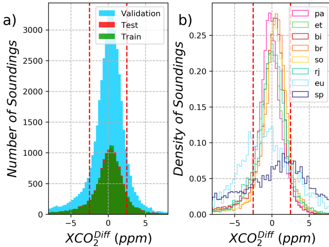
580 Figure 2 a) Histogram of the bias between coincident TCCON and OCO-2 retrievals XCO_2^{Diff} (Eq. 3), for the three datasets. The red dashed lines represent the boundary between setting the classification of the data. b) Same as plot 'a)' but shows the density of soundings for each of the sites.
