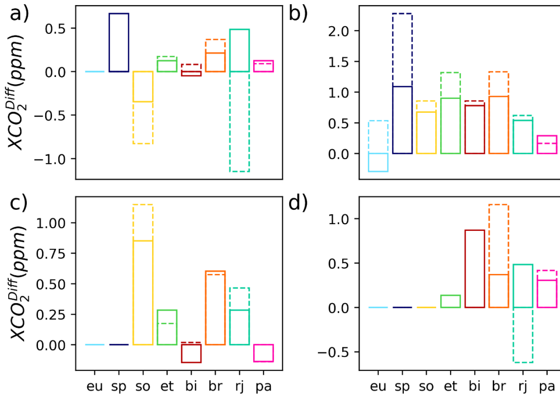
595 Figure 5 The bias at each site for the different seasons when the NN filter (bars with solid lines) and qc_flag (bars with dashed lines) is used to filter the OCO-2 retrievals in the validation data set. a) Spring (March, April, May). b) Summer (June, July, August). c) Fall (September, October, November). d) Winter (December, January, February). Note the different y-axis ranges for each plot. Note that bars that show a bias of zero are due to no data rather than a bias of zero.
