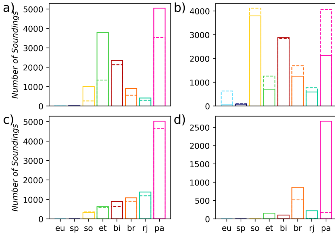
605 Figure 7 Same as Figure 5 but shows the number of soundings that pass each filter at each site for the different seasons. a) Spring (March, April, May). b) Summer (June, July, August). c) Fall (September, October, and November). d) Winter (December, January, February). Solid bars indicate the NN filter, and dashed bars indicate the original B10 qc_filter.
