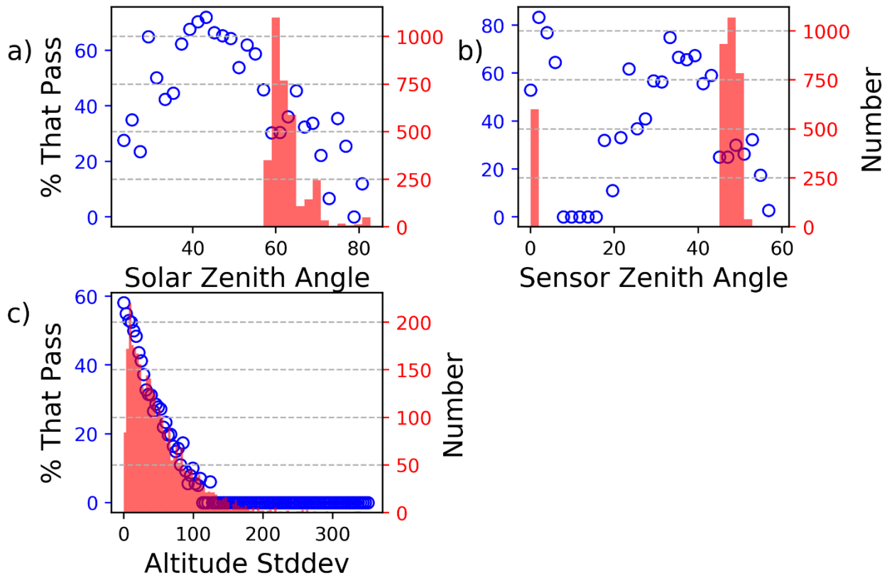
590 Figure 4 The percentage of data that passes the NN filter (blue dots) for a given solar zenith angle (a), sensor zenith angle (b) and altitude standard deviation (stddev) (c). The bars are the histograms of the OCO-2 soundings coincident with the Eureka TCCON data.
