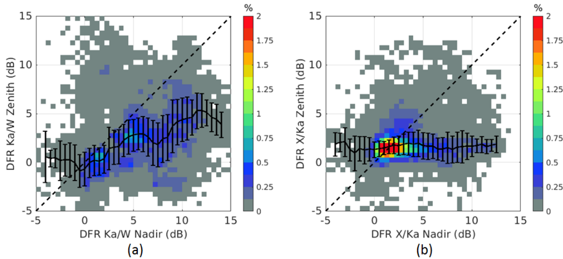
Figure 5: Scatterplots of (a) DFR Ka/W and (b) DFR X/Ka at 245 m above and below the aircraft from the 22 November flight. The data grid is 0.5 dB. The dashed black line is the 1:1 line. The solid black lines are the mean curve and the one standard deviation error bars.
