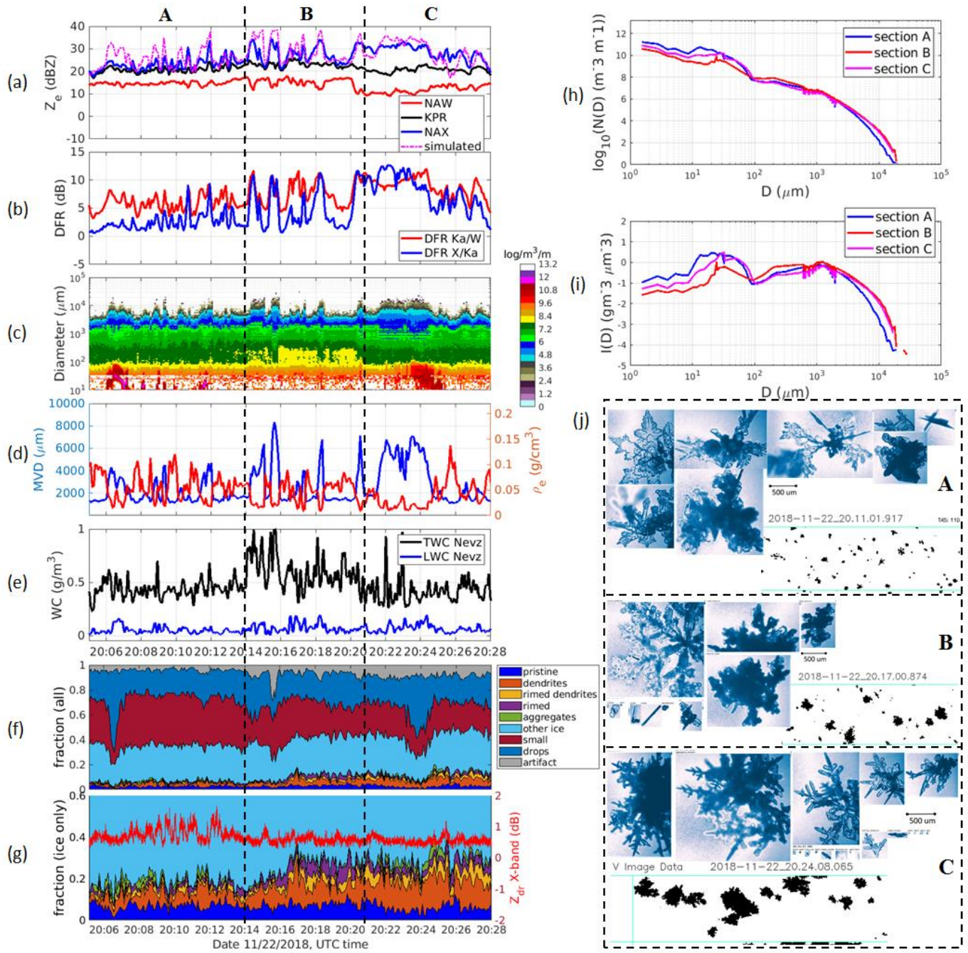
Figure 12: Similar to Fig. 10 but for flight segment 20:05 UTC – 20:28 UTC.
