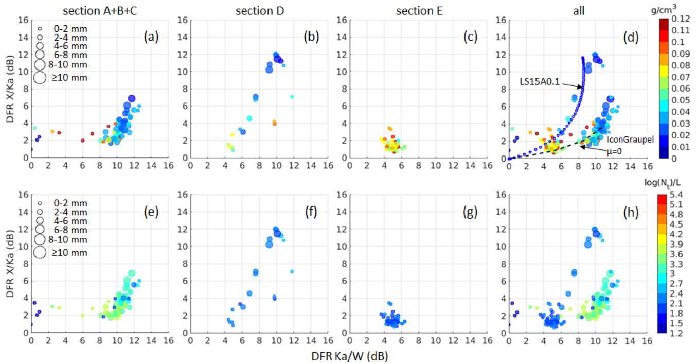
Figure 11: DFR scatterplots for the 1938-2000 UTC segment in the November 22 flight. Data points are coloured by the effective bulk density ( \rho_e ) (a-d) and by the total concentration ( N_t ) (e-h). The dot size is proportional to the calculated MVD. In panel (d), the blue line is for riming model A with effective liquid water path of 0.1 \text{ kg m}^{-2} (Leinonen and Szyrmer, 2015) and the black line is for a graupel model from Fig. 2.
