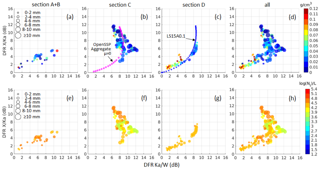
485 Figure 15: Similar to Fig. 14 but for flight segment 20:05 UTC – 20:28 UTC. The magenta line (in panel (b)) is for the aggregation scattering model (Kuo et al., 2016)) and the blue line (in panel (c)) is for riming model A with effective liquid water path of 0.1 \text{ kg m}^{-2} (Leinonen and Szyrmer, 2015)
