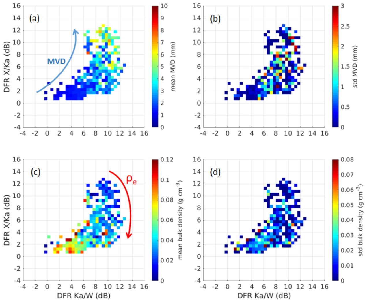
490 Figure 16: (a) Mean MVD; (b) standard deviation (std) of MVD; (c) mean \rho_e ; and (d) std of \rho_e calculated from all the data points (573 samples) analysed in three study cases of the 22 November flight. The data are binned onto a grid with grid size of 0.5 dB in both axes. The mean and standard deviation are computed from the data within the bin.
