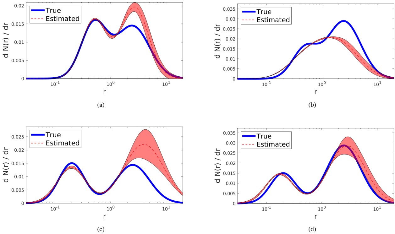
Figure 6. Reconstructions obtained by running the inversion algorithm with a bimodal distribution, when data are generated by a bimodal distribution. Different panels from (a) to (d) correspond to different parameters characterizing the bimodal distributions: the respective parameter values are given in Table 2 (section “Bimodal case”).
