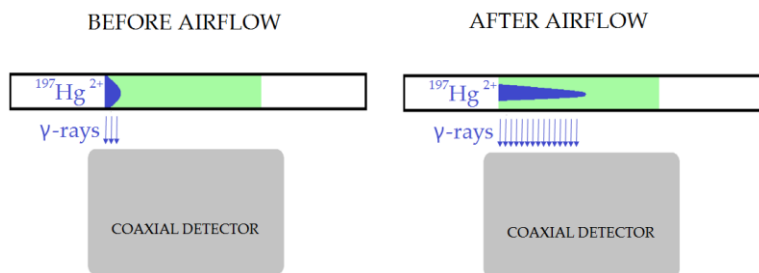
Figure 5: Effect of radiotracer distribution change along the trap on the activity measurement after exposure of KCl sorbent traps to air flow (not shown depicted to scale).
