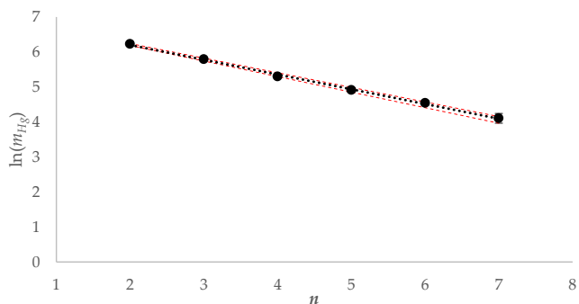
Figure 11: Example \ln(m_{Hg}) against extraction number ( n ), linear regression for KCl at 5°C (red error bars \pm 1 u_c ( k = 1 ), 1).
