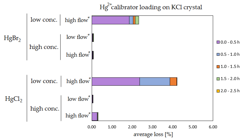
325 Figure 6: Results of the stability test for the ^{197}\text{Hg}^{2+} (radiotracer) spike on KCl crystal. Low concentrations were loaded with less than 1 ng Hg per time period and high concentrations were loaded with more than 50 ng of Hg per time period. Low air flow experiments were performed with 100 \text{ mL min}^{-1} air flow while high air flow experiments were performed with 400 \text{ mL min}^{-1} flow. Asterisks mark the results that only have the first 4 time periods.
