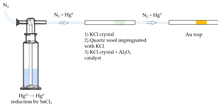
Figure 1: Scheme of the experimental setup for testing the extent of undesirable \text{Hg}^0 retention on three different KCl sorbent trap designs (not shown depicted to scale).
