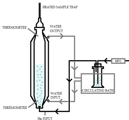
Figure 3: Henry's law extractor stripping vessel arrangement.
