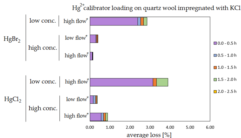
340 Figure 9: Results of the stability test for the calibrator loading of ^{197}\text{Hg}^{2+} (radiotracer) on quartz wool impregnated with KCl. Low concentrations were loaded with less than 1 ng Hg per time period and high concentrations were loaded with more than 50 ng of Hg per time period. Low air flow experiments were performed with 100 \text{ mL min}^{-1} air flow while high air flow experiments were performed with 400 \text{ mL min}^{-1} flow. Asterisks mark the results that only have the first 4 time periods.
