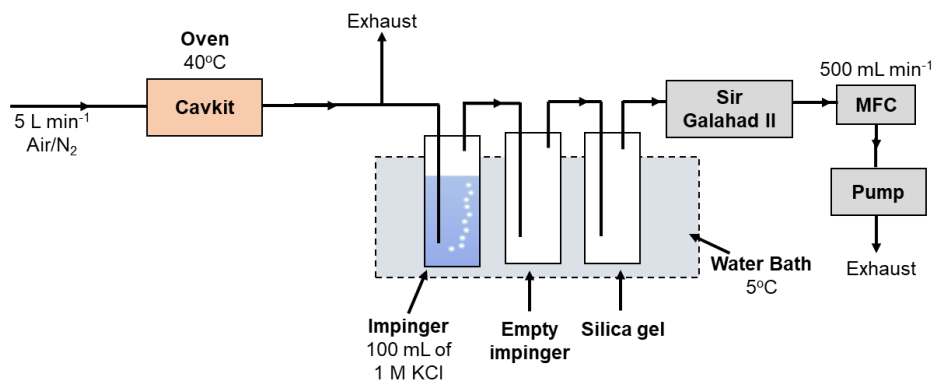
Figure 4: Experimental arrangement for KCl trapping experiments.
