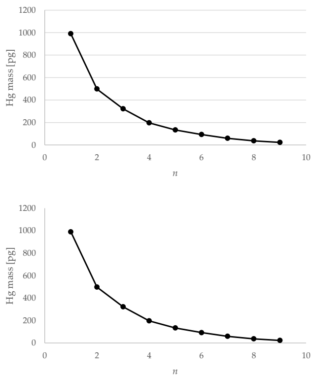
Figure 10: Example m_{(Hg)} against extraction number ( n ) for 1 mol L -1 KCl at 5°C.
