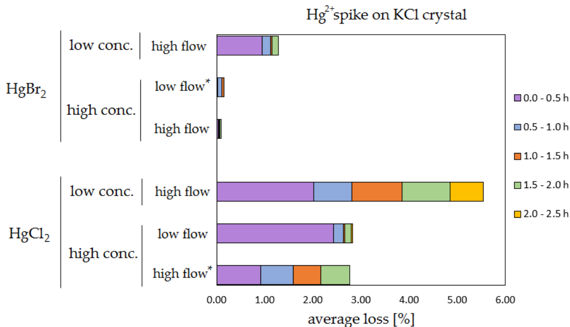
290 Figure 6: Results of the stability test for the ^{197}\text{Hg}^{2+} (radiotracer) spike on KCl crystal. Low concentrations were loaded with less than 1 ng Hg per time period and high concentrations were loaded with more than 50 ng of Hg per time period. Low air flow experiments were performed with 100 \text{ mL min}^{-1} air flow while high air flow experiments were performed with 400 \text{ mL min}^{-1} flow. Asterisks mark the results that only have the first 4 time periods.
