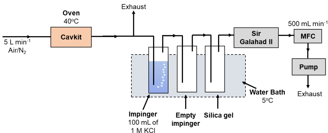
Figure 4: Experimental arrangement for KCl trapping experiments.
