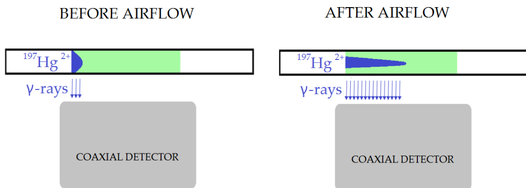
280 Figure 5: Effect of radiotracer distribution change along the trap on the activity measurement after exposure of KCl sorbent traps to air flow (not depicted to scale).
