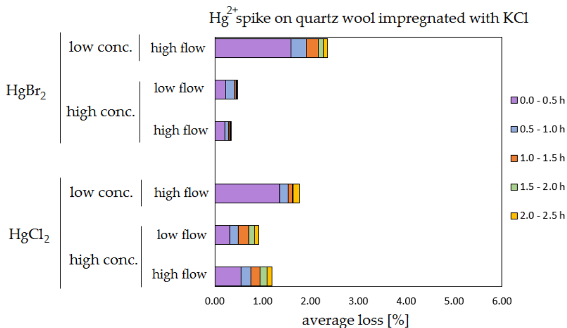
300 Figure 8: Results of the stability test for the ^{197}\text{Hg}^{2+} (radiotracer) spike on quartz wool impregnated with KCl. Low concentrations were loaded with less than 1 ng Hg per time period and high concentrations were loaded with more than 50 ng of Hg per time period. Low air flow experiments were performed with 100 \text{ mL min}^{-1} air flow while high air flow experiments were performed with 400 \text{ mL min}^{-1} flow.
