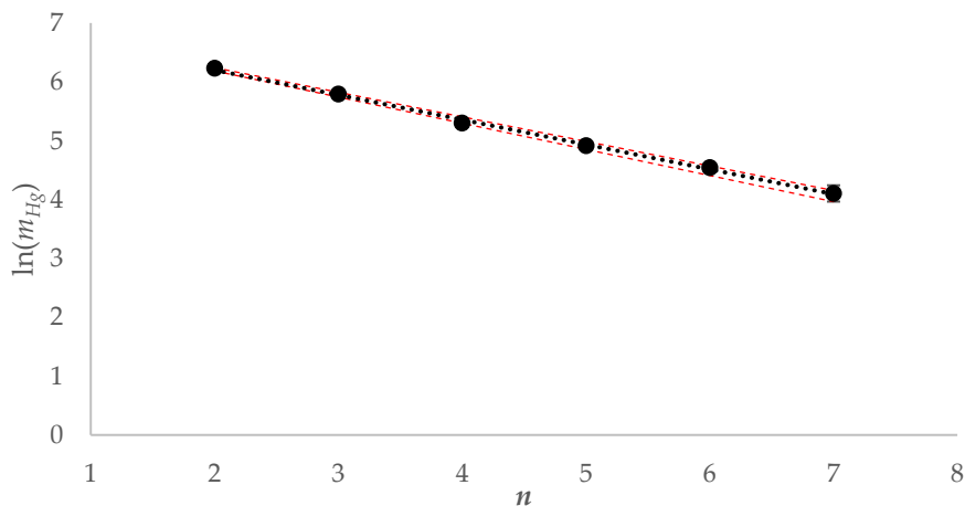
Figure 11: Example \ln(m_{Hg}) against extraction number ( n ), linear regression for KCl at 5°C (red error bars \pm 1 u_c [ k = 1 ]).
