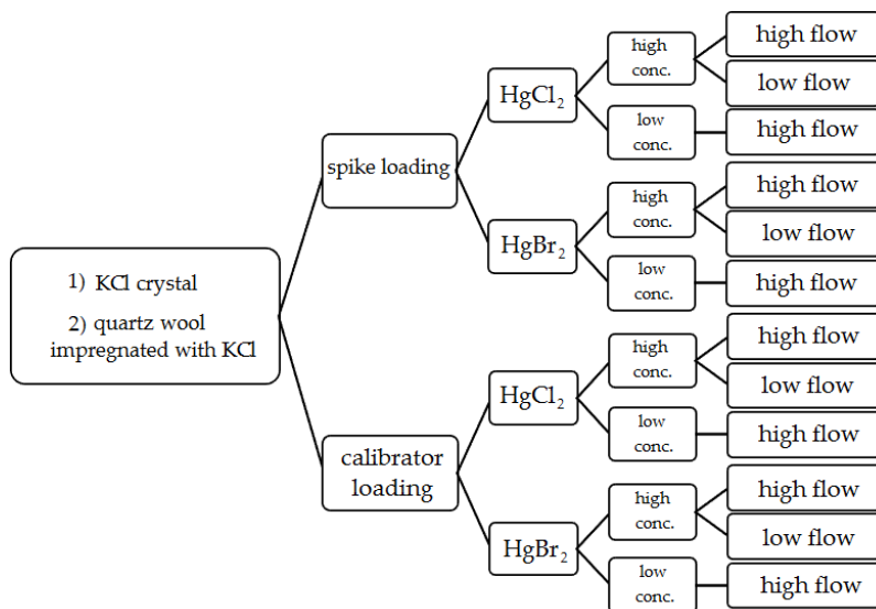
160 Figure 2: Variations of performed experimental conditions for \text{Hg}^{2+} stability on KCl sorbent traps during exposure in ambient air flow.
