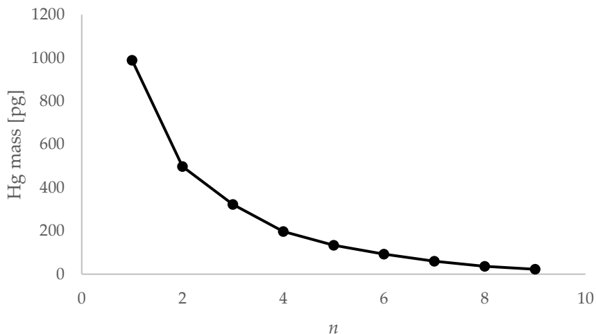
Figure 10: Example m_{(Hg)} against extraction number ( n ) for 1 mol L -1 KCl at 5°C.
