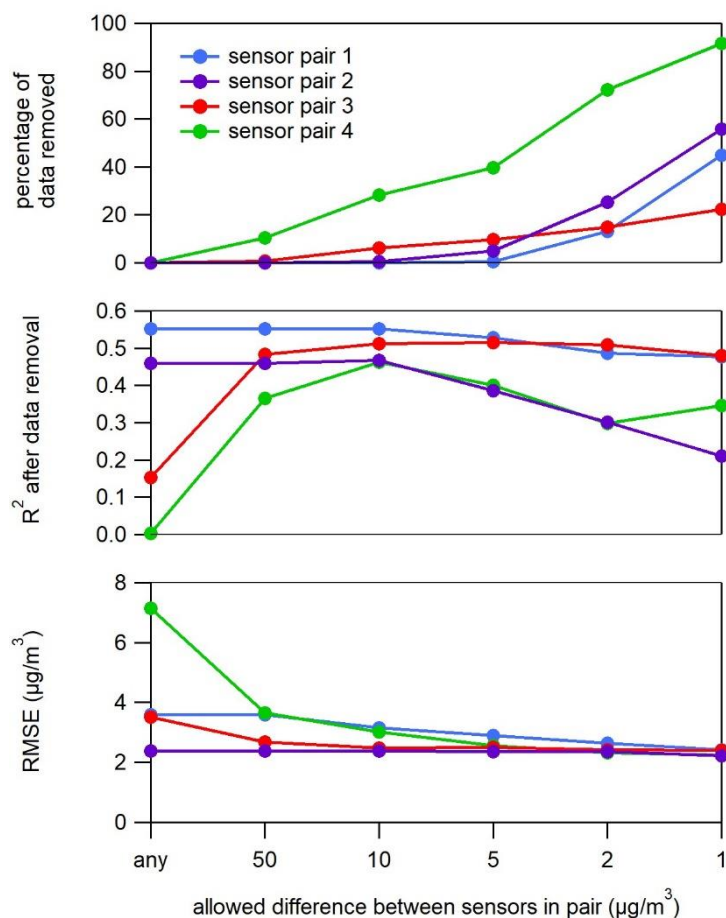
Figure 1. The eight sensor replicas were divided into four pairs with different measurement agreement requirements for the data from the sensors in each pair ( first averaged to 1-hour intervals ). The x-axis shows the allowed difference between paired measurements. The top figure shows the percentage of data that is removed from the sensor pair for different data agreement requirements. The bottom-middle figure shows how R^2 between the sensor pair (average of the pair) and reference measurements changes as when these disagreeing data points are removed. The bottom figure shows how RMSE is impacted as disagreeing data points are removed.
