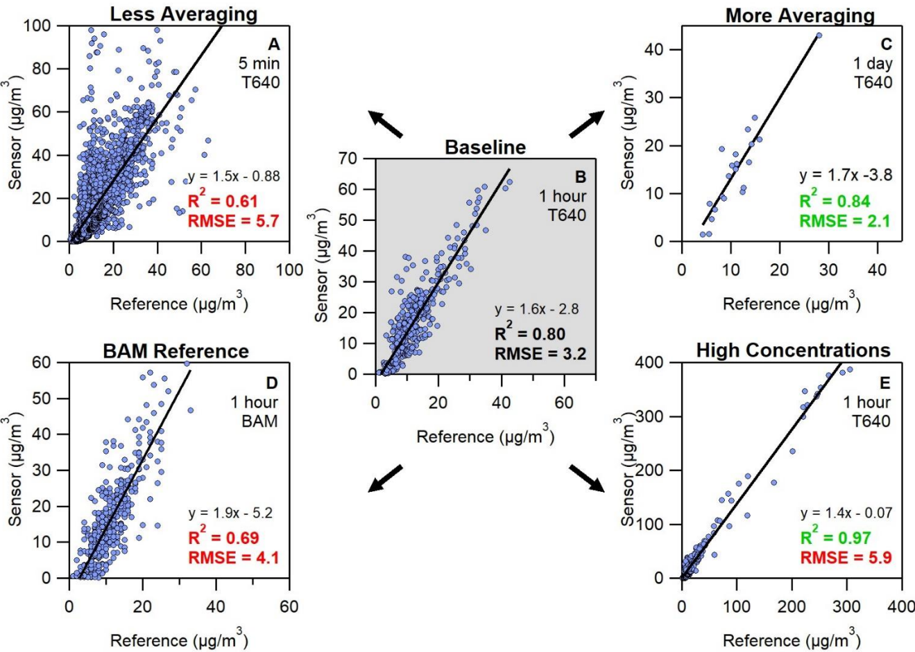
Figure 3. The changes to R^2 and RMSE from a baseline condition depending on evaluation conditions. (B) shows the baseline of 1-hour averaged data, T640 as a reference instrument, and without three days of high concentrations. (A) and (C) show the impact of less and more data averaging, respectively. (D) shows the impact of switching to the BAM instead of the T640. (E) shows the effect of high concentration by including three additional days during which higher concentrations were observed.
