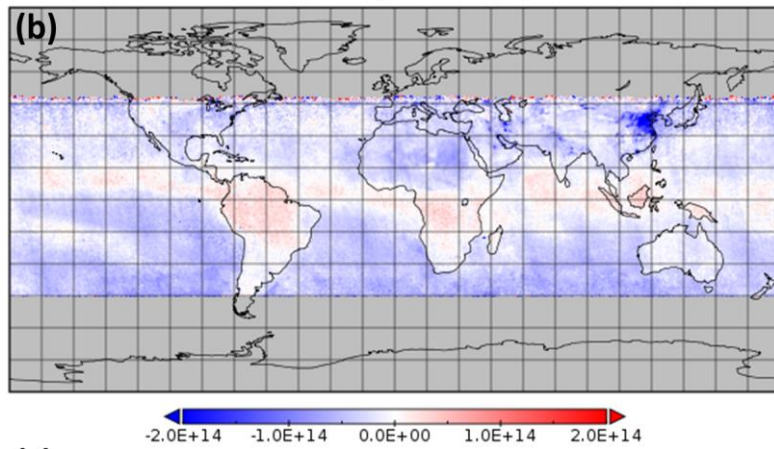
CHOCHO SCD differences (molec.cm-2) - with-w/o Pukite
