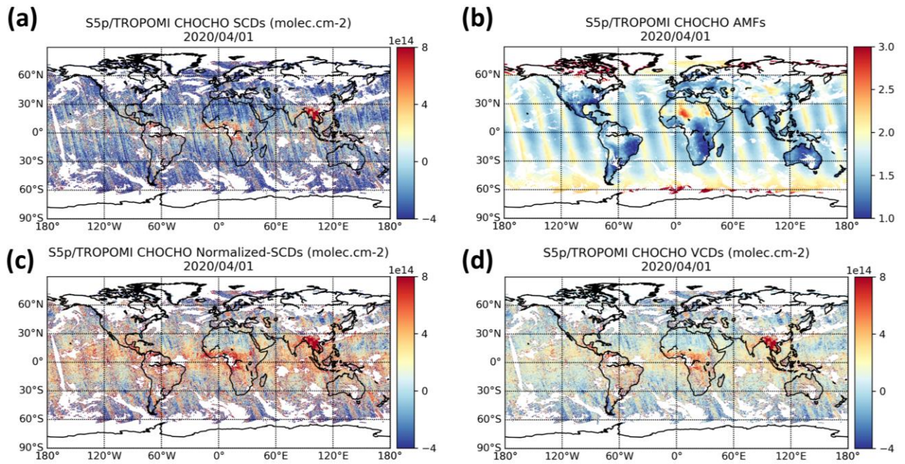
Figure 1: Illustration of the different glyoxal algorithmic steps for one day of TROPOMI data (01/04/2020). (a) Glyoxal SCDs retrieved from the DOAS spectral fits; (b) Glyoxal AMFs; (c) Glyoxal normalized-SCDs resulting from the background correction procedure; (d) Final retrieved glyoxal VCDs. The data has been gridded at the spatial resolution of 0.25^\circ .
