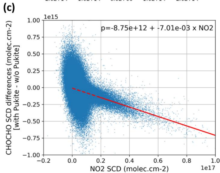
Figure 4 : (a) Monthly mean NO 2 SCDs retrieved from TROPOMI data in December 2019. Panel (b) illustrates the CHOCHO SCD absolute differences (molec/cm 2 ) due to the incorporation of the Pukite et al. (2010) cross-sections in the DOAS spectral fit and panel (c) shows the correlation between those differences and the NO 2 SCDs. The red line corresponds to a linear regression fit through all points with NO 2 SCD larger than 2x10 16 molec/cm 2 .
