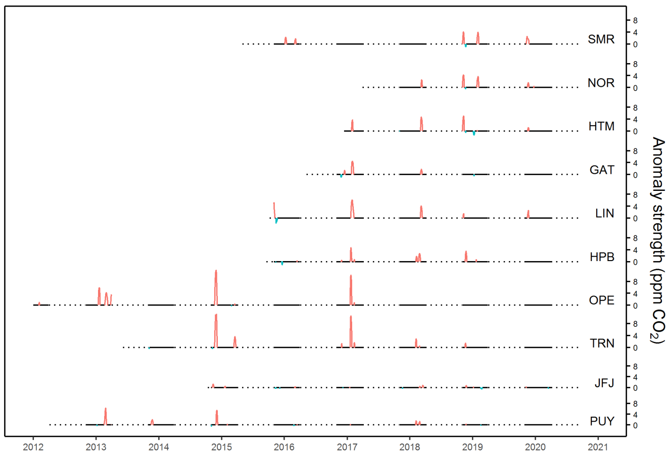
Figure 6: Positive (red) and negative (blue) SSAs in the complete CO 2 records of each site. The anomaly strength refers to the difference between the 30-day LOESS curve and the boundary of the \pm 2\sigma_{30} -envelope.
