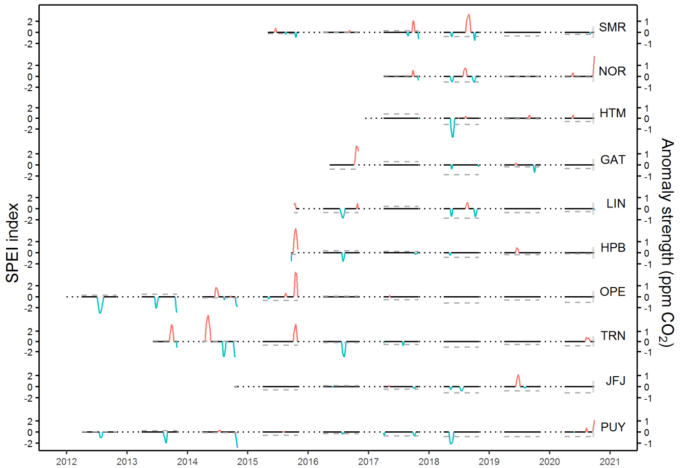
Figure 9: Positive (red) and negative (blue) 90-day seasonal CO 2 anomalies. April–October average SPEI values are indicated by the dashed gray lines. The gray bar on the right end of the plots indicates the standard deviation of summer SPEI values from 1999–2020.
