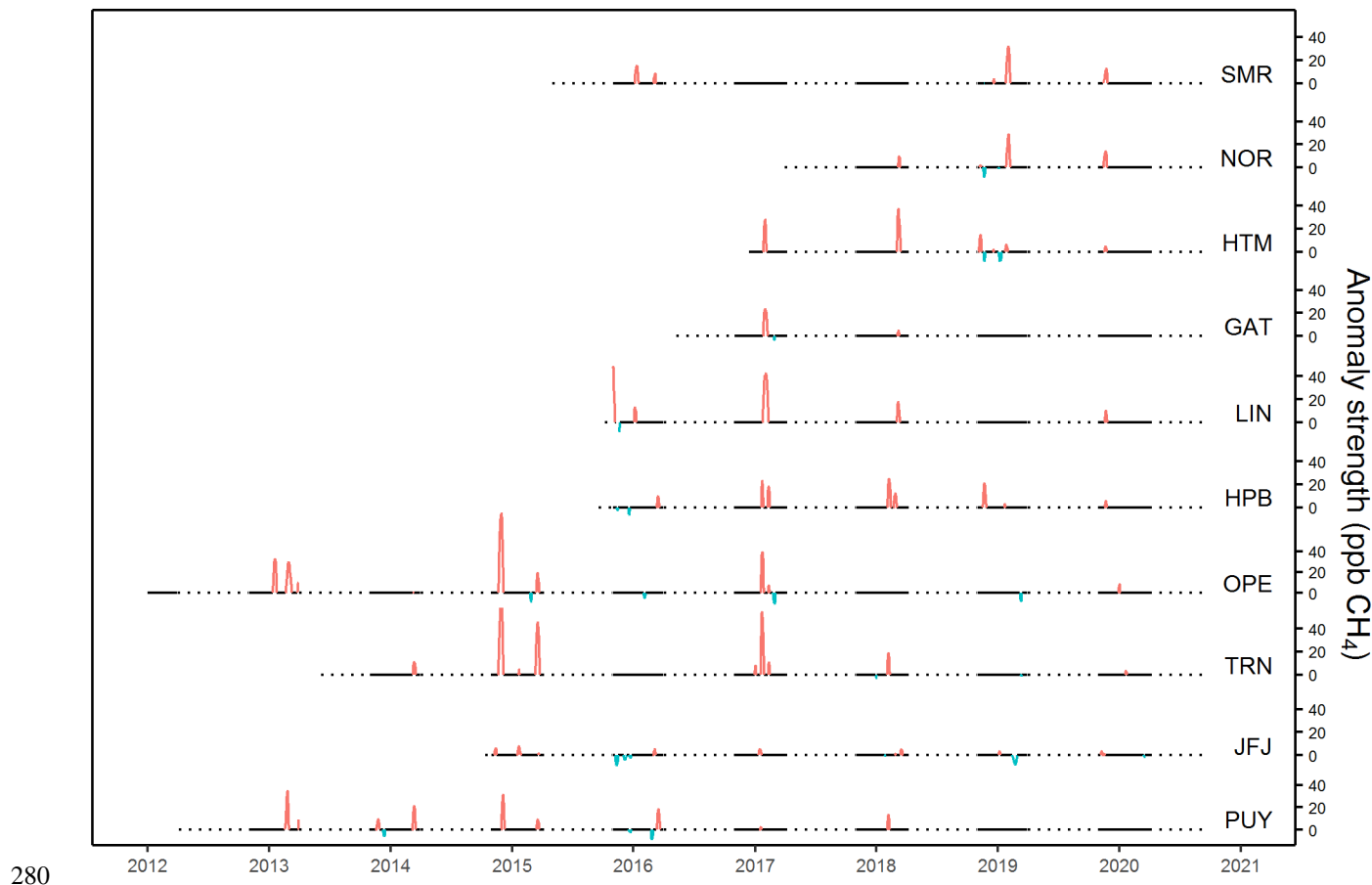
Figure 7: Positive (red) and negative (blue) SSAs in the complete CH 4 records of each site.
