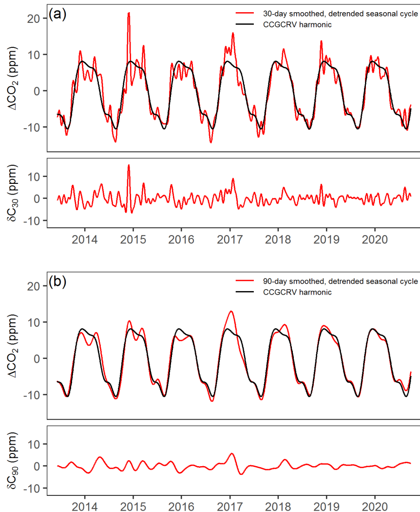
Figure 3. The smoothed, detrended seasonal cycle at TRN (red) extracted using (a) 30- and (b) 90-day short-term filters of the CCGCRV function residuals. \Delta\text{CO}_2 represents the calculated mean seasonal variation in \text{CO}_2 , excluding the long-term trend.
