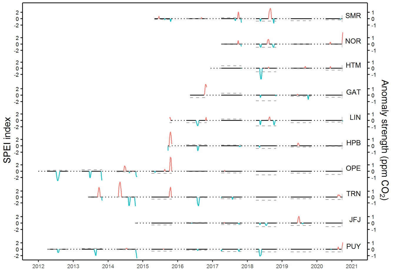
Figure 9: Positive (red) and negative (blue) 90-day seasonal CO 2 anomalies. April–October average SPEI values are indicated by the dashed gray lines. The gray bar on the right end of the plots indicates the standard deviation of summer SPEI values from 1999–2020.
