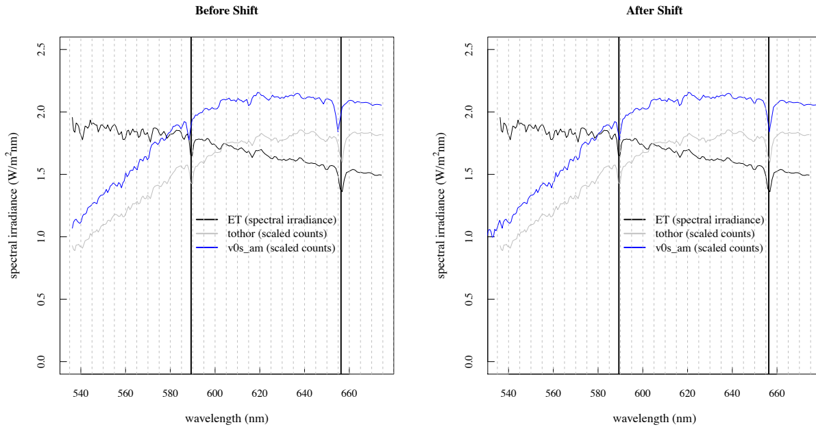
480 Figure 2: The average of nine spectra near solar noon appears as the blue line; the extraterrestrial spectrum (ET) at RSS resolution is the black line (units on y-axis refer to the ET), and the gray line is the carefully determined spectrum used as the standard total horizontal spectrum that is compare to all RSS data. The blue spectrum in the left panel is shifted shortward by two pixels and the right panel shows the shift-corrected spectrum. The two absorption lines are in the solar spectrum since they also appear in the ET spectrum; these are the sodium doublet 589.0/589.6 nm and the hydrogen alpha line 656.3 nm.
