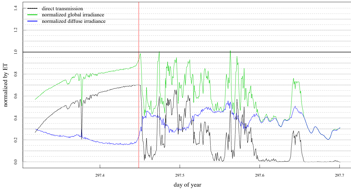
515 Figure 8: Plot of the direct normal transmission and the normalized global and diffuse irradiances near 500 nm for 24 October 2009 at the ARM site in northern Oklahoma. The vertical red line marks the time of the measured spectra in Figure 7. The direct transmission appears unaffected by nearby clouds, but the normalized diffuse irradiance and, therefore, the normalized global diffuse irradiance are enhanced over the clear-sky values explaining the effect of apparent normalized global irradiance greater than 100% in Figure 7.
