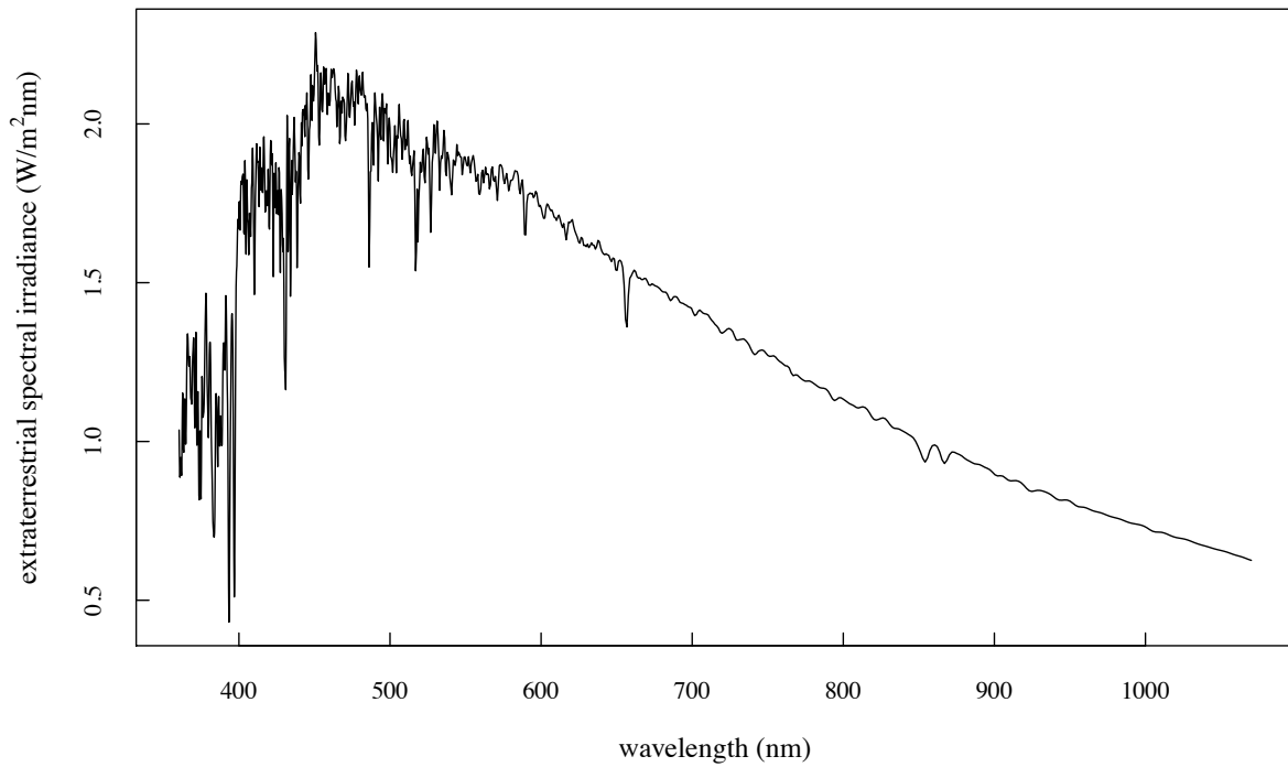
Figure 3: Extraterrestrial solar spectrum used for this paper using RSS slit function applied to Kurucz high-resolution calculated ET solar spectrum, then scaled to the Gueymard low resolution ET solar spectrum, which is regarded as our best estimate of absolute irradiances.
