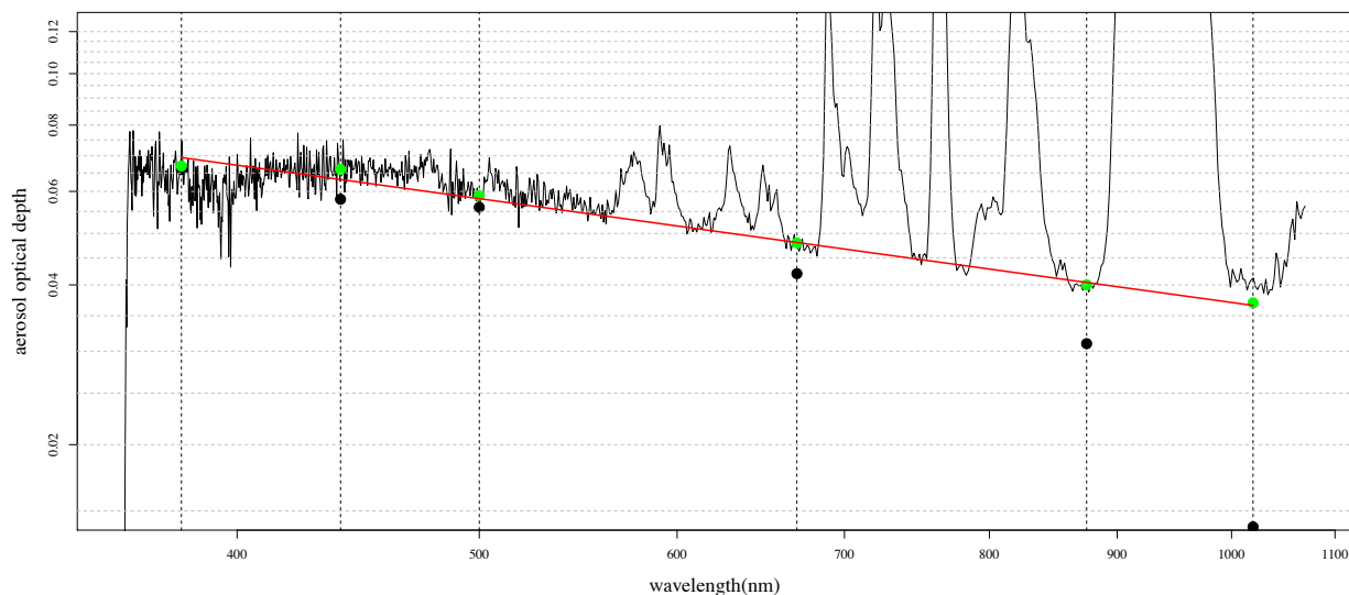
535 Figure 10: RSS aerosol optical depth versus wavelength at 11:45 local standard time at the ARM central facility in northern Oklahoma. The vertical lines are drawn at the wavelengths used in the CIMEL sunphotometers employed by AERONET for measuring AODs in this part of the spectrum. The O 2 and H 2 O bands have been truncated at 0.12 optical depth to better see the aerosol wavelength dependence. Approximated RSS AOD (green dots) versus wavelength for pixels at AERONET wavelengths. Least squares fit to the RSS points yields an Angstrom exponent equal to 0.52. The filled 540 black dots are the AERONET points taken 2.5 minutes after the RSS data. Except for 1020 agreement is within 0.01 AOD. The 1020 nm (green) point for the RSS is lower by 0.003 because an additional correction was made for water vapor at that wavelength.
