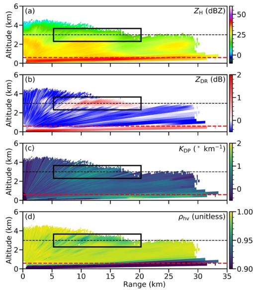
505 Figure 6. Height-range plots of observed (a) Z_H , (b) Z_{DR} , (c) K_{DP} and (d) \rho_{HV} from the RHI scan at 8:37 UTC on 13 February 2018 during the PICASSO field campaign. The red dashed line denotes the 0^\circ\text{C} level, while the black dashed line denotes the approximate flight altitude of FAAM during the scan. The black polygon denotes the region that has enhanced Z_{DR} and K_{DP} , and reduced \rho_{HV} .
