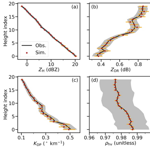
470 Figure 4. Profiles of (a) Z_H , (b) Z_{DR} , (c) K_{DP} and (d) \rho_{HV} for synthetic observations (black line) calculated from the ice cloud properties given in Fig. 5, and for the mean of forward simulations from the ensemble (red dots). Grey shading denotes the observational 475 uncertainties given in Table 3, while error bars in orange denote retrieval uncertainty calculated as the one-standard deviation spread of the ensemble simulations.
