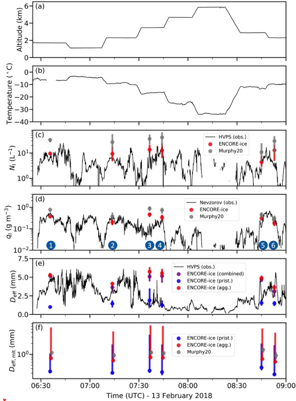
595 Figure 9. Time series of (a) flight altitude, (b) temperature, observed and retrieved (c) total ice number concentration, (d) ice water content, (e) effective mean diameter using the maximum particle dimension as the size descriptor, and (f) effective mean diameter using the equivalent melted diameter as the size descriptor. Retrieval from ENCORE-ice and Murphy20 empirical relationships are denoted by dots, explained by detailed legends. The dots represent the median of retrieval from all collocated gates, and the vertical bars denote the range between the 25th and 75th percentiles. Note that the counting uncertainty in total ice number concentration in (c) is plotted but too small to see. All calculations are based on the size range of HVPS observations, except Murphy20 retrievals in (c) and (d). For convenience, we index six retrieval clusters from 1 to 6 as shown in (d).
