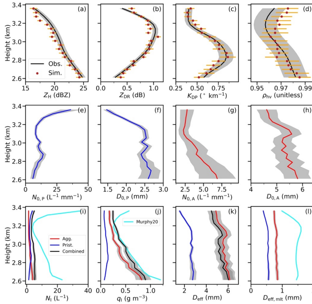
515 Figure 8. Retrieval performance for a radar ray at 8:37:39 UTC. Observed and forward simulated profiles of (a) Z_H , (b) Z_{DR} , (c) K_{DP} and 520 (d) \rho_{HV} . The shading in (a)–(d) represent the observational uncertainty. The red dots represent the mean of the ensemble simulations, and the error bars represent one standard-deviation in forward simulations. (e)–(j) represent the retrieved mean normalized pristine ice number concentration, pristine ice normalization diameter, normalized aggregate number concentration, aggregate normalization diameter, the total number concentrations, and the total ice water content, respectively. (k) and (l) represent the individual and combined effective mean diameters using the maximum particle dimension and the equivalent melted particle size as the size descriptor, respectively. The shading in (e)–(l) represent one standard deviation uncertainty in retrieval. For comparisons, retrievals from Murphy20 are co-plotted in (i), (j) and (l).
