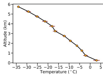
510 Figure 7. A temperature profile composed from aircraft in-situ data during 6–9 UTC on 13 February 2018. Data between 6:33:30 – 6:39:20 UTC were unphysical (see Fig. 9b) and thus excluded. The error bars represent one standard deviation of sampled observations.
