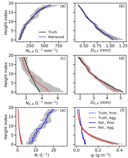
480 Figure 5. Profiles of (a) normalized number concentration and (b) normalization diameter for pristine ice, (c) normalized number 485 concentration and (d) normalization diameter for aggregates. (e) represents the total number concentrations and (f) represents ice water contents of pristine ice and aggregates. Truth is denoted by black solid lines in (a)–(d), and by dashed lines in (e) and (f). The retrieved ensemble means are denoted by solid blue and red lines with shading that represents the one-standard deviation spread of the ensemble members. The habit of pristine ice is plate in this experiment.
