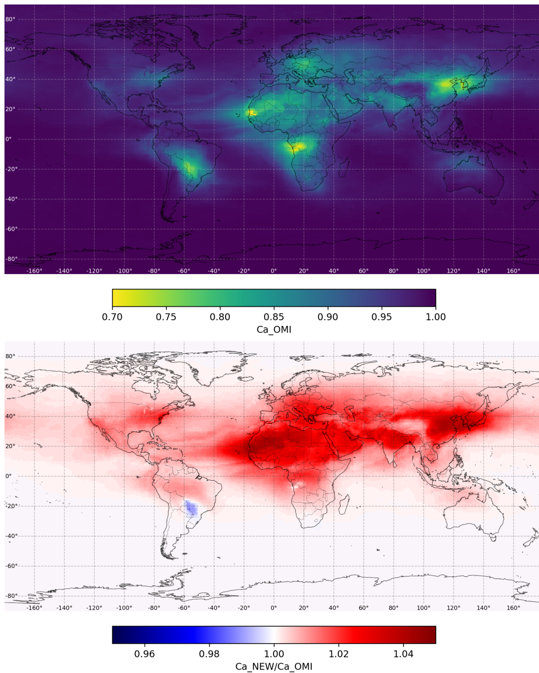
Figure 5. Same as Figure 4, but both SZA and aerosol climatology corresponds to June conditions
