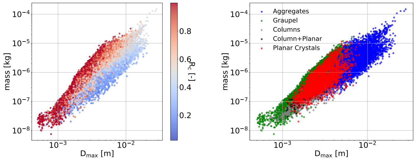
Figure 5. m(D_{\max}) scatter plots for the data of a field campaign, named Davos 2015 , taking place in the Swiss Alps in 2015 and 2016. Left: data color-coded according to riming index R_c of Praz et al. (2017). Right: data color-coded according to the hydrometeor classes, also of Praz et al. (2017).
