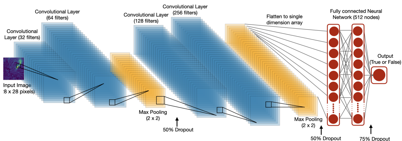
Figure 1. Simplified schematic of the convolutional neural network architecture to identify \text{NO}_2 plumes. See main text for further details.
