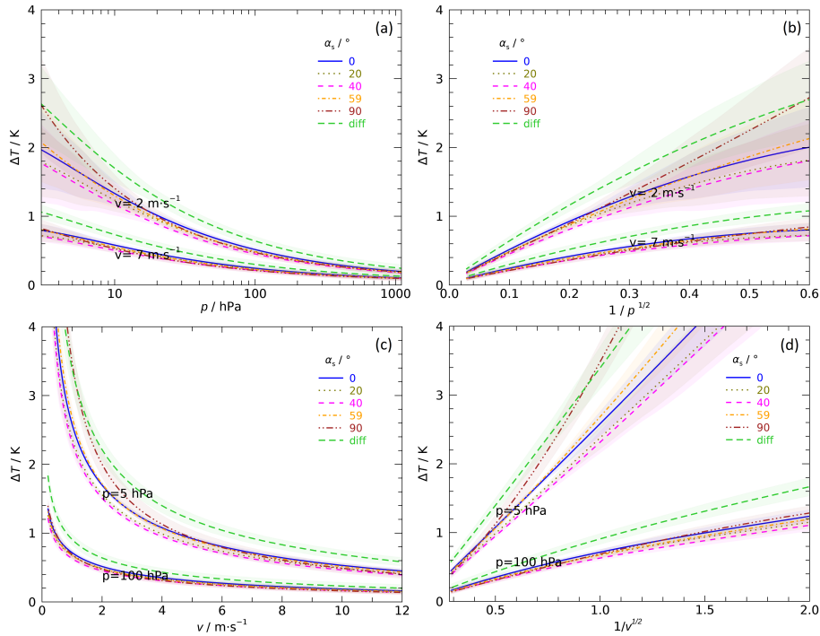
Figure 14. Comparison of the solar temperature error for different various radiation incidence angles ( \alpha_s ). \Delta T from Eq. (5) is normalised, i.e. linearly scaled, for each ( \alpha_s ) to an irradiance equivalent to the solar constant ( 1361 \text{ W m}^{-2} ) beforehand. Left Upper row: Examples for ventilation levels of 2 \text{ m s}^{-1} and 7 \text{ m s}^{-1} ; (a) pressure as x-axis; logarithmic scale for better visibility, (b) plot vs. 1/p^{1/2} . Lower row: Examples for pressure levels of 5 hPa and 100 hPa; (c) ventilation as x-axis; (d) plot vs. 1/v^{1/2} . Shaded areas around the graphs denote 1\sigma -uncertainty estimates. The grey shading in the background indicates the range of prevailing ventilation velocities in soundings.
