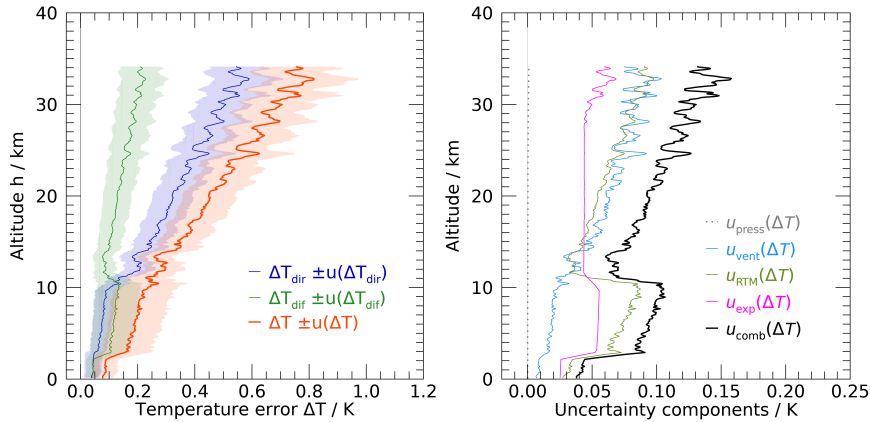
Figure 18. Left: Example for the estimated solar radiation error of temperature measurements (Lindenberg, 2020-06-11, 12:00 UTC). Red: Overall overall bias, blue: component from direct radiation, green: component from diffuse radiation; shaded areas indicate uncertainties ( k = 1 ). Right: Uncertainty components ( k = 1 ) associated with pressure, ventilation speed, radiation model, and laboratory experiments.
