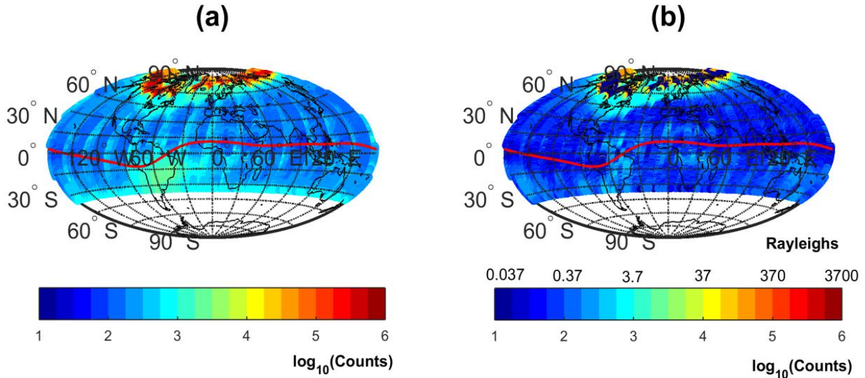
160 Figure 7: The global count (left) and brightness (right) of the 135.6nm nightside channel from 7 to 11 December 2017. The brightness is without red-leak and the effect of dark count. The red solid line indicates the magnetic dip equator.
