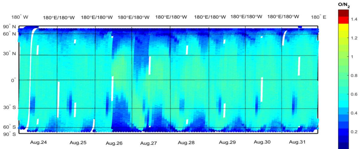
Figure 12: Column O/N_2 from GUVI around the magnetic storm of Aug.26, 2018.
