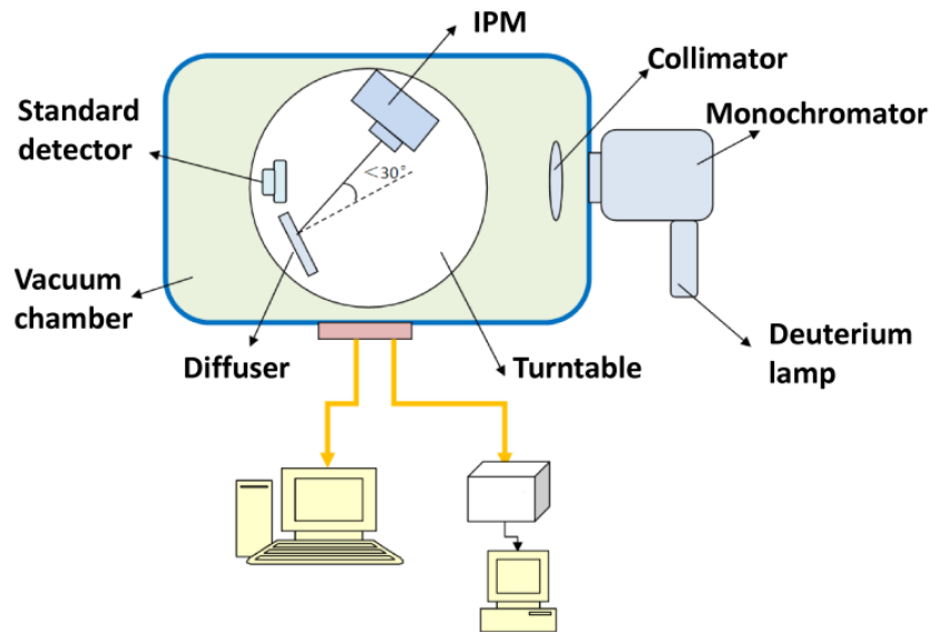
Figure 2: The optical calibration facility at ground
