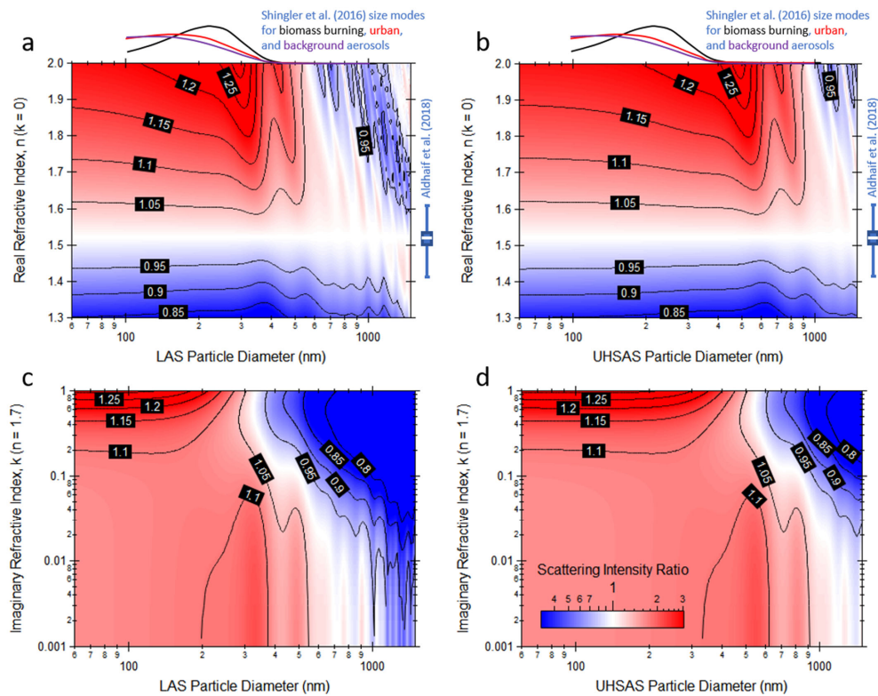
870 Figure 1: Mie theory calculations of size-resolved particle scattering normalized to that for ammonium sulphate ( 1.52+0i ) at the LAS 875 laser wavelength of 633 nm (a, c) and the UHSAS laser wavelength of 1054 nm (b, d). In panels a and b, the imaginary part of the refractive index is held constant at zero, while for panels c and d, the real part of the refractive is held constant at 1.7. The coloured shading represents the ratio of the theoretical particle scattering cross section, while the contours approximate the expected sizing ratio, which is assumed to be equal to the sixth root of the scattering cross section ratio (reasonable for diameters below 300-600 nm). Average number size distribution modes for relevant atmospheric aerosol types from Shingler et al. (2016) are shown on top of panels a and b to illustrate the typical atmospheric aerosol size range, while the range of real RIs reported by Aldhaif et al. (2018) are shown to the right of these panels to illustrate the typical range of atmospherically-relevant real RIs.
