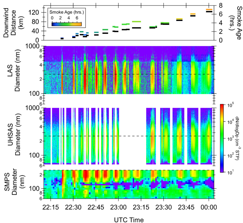
Figure 9: Timeseries of the measured aerosol size distributions from the DC-8 on the 3 August 2019 Williams Flats Fire in the state of Washington, USA, during FIREX-AQ. The top panel shows the approximate smoke age and downwind distance, corresponding to each plume transect as shown in Figure 8. The three lowest panels are the measured size distribution expressed as dN/d\log D_p ( \text{cm}^{-3} STP). The horizontal dashed line denotes the upper size limit of the SMPS, which is plotted on a different size scale from the LAS and UHSAS. Reported sizes are for dry particles ( \text{RH} < 40\% ). Local time is Pacific Daylight Time (UTC-7).
