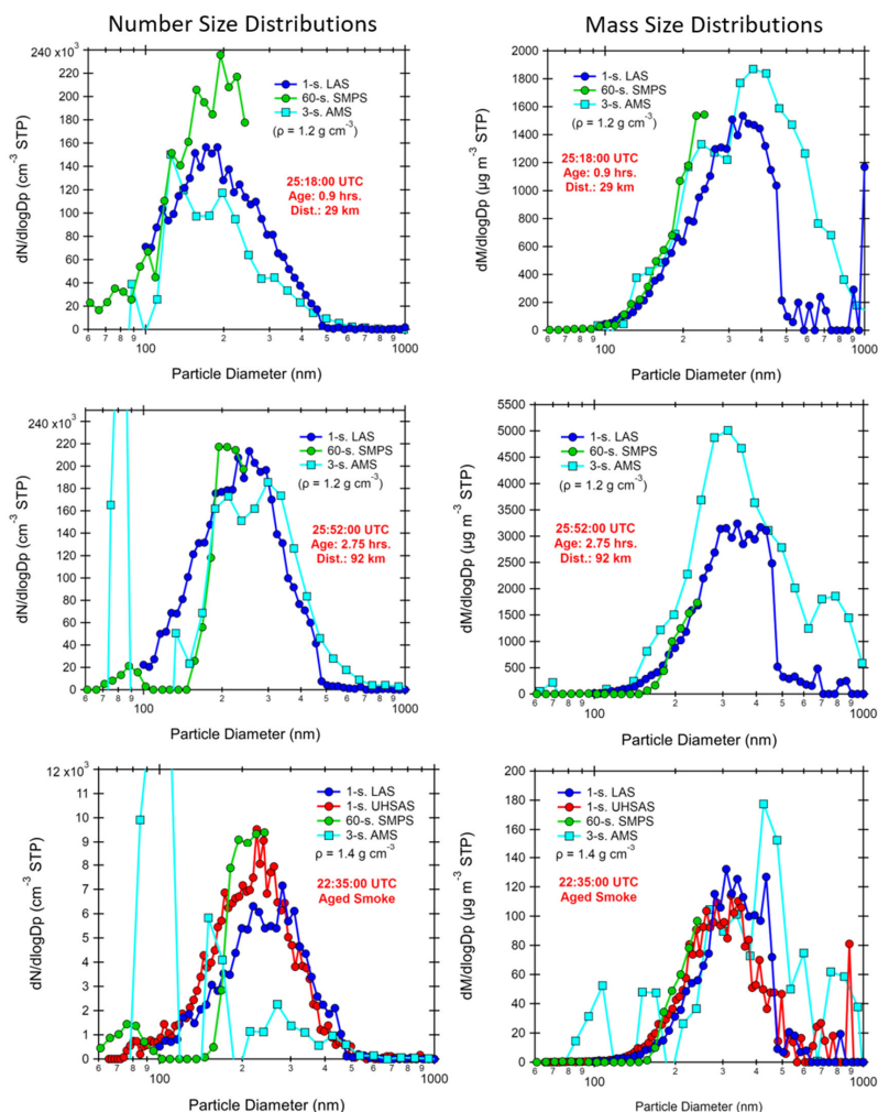
Figure 11: Comparison of the size distributions measured by the AMS, LAS, UHSAS, and SMPS at three downwind distances from the Williams Flats Fire in the state of Washington, USA, during the 7 August 2019 FIREX-AQ flight, including smoke sampled much farther afield. Mass distributions are computed for the LAS, UHSAS, and SMPS assuming spherical particles and using the aerosol density estimated from the mass spectrometer, while the calculation is applied in reverse to compute AMS number distributions. This density is also used to convert the AMS vacuum aerodynamic diameters to spherical-equivalent diameters. Reported sizes are for dry particles (RH < 40%).
