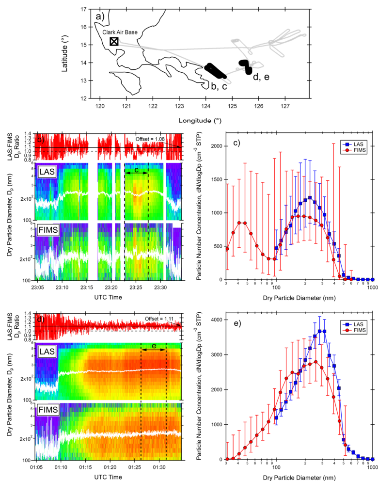
Figure 12: Comparison of the LAS and FIMS aerosol accumulation mode size distributions for aged biomass burning plumes encountered during CAMP 2 EX-CAMP 2 Ex research flight on 16-17 September 2019 east of the Philippines . Panel a shows the flight track in gray with bolded regions indicating the plume encounters. Panels b and d show the size distribution time series for each instrument with the white trace denoting the count mean diameter (CMD) of the size distribution. Also shown is the ratio of the CMDs for the LAS and FIMS. Panels c and e are the geometric mean (* one geometric standard deviation) of the aerosol size distributions for level flight legs within the most intense portion of the plume intercept (denoted by the vertical dashed lines in Panels b and d).
