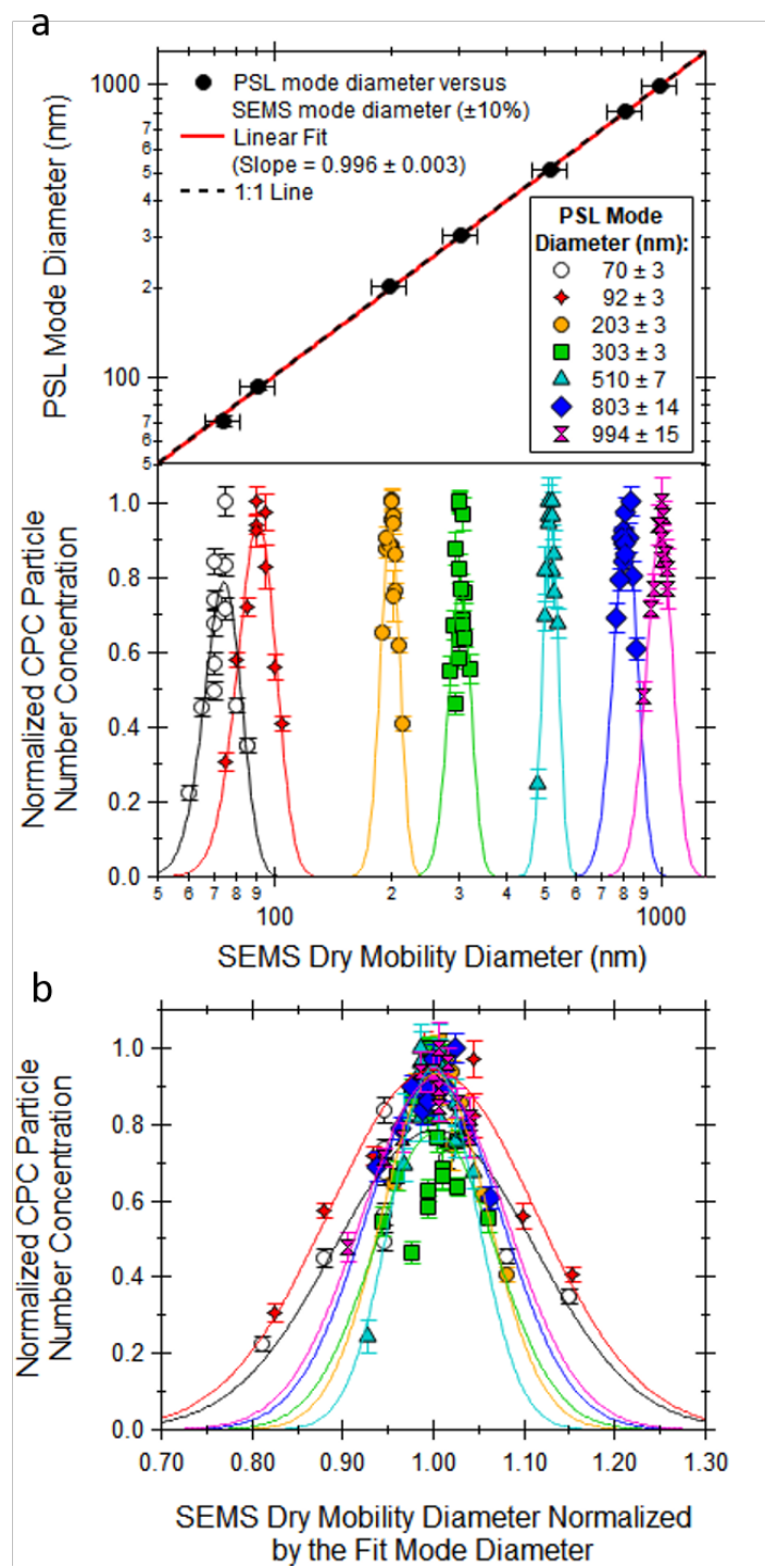
Figure 3: SEMS DMA sizing verification with NIST-traceable polystyrene latex spheres (PSLs) size standards. Panel a compares the PSL mode and SEMS fit mode mobility diameters (top) and the fits to the CPC concentration peaks (bottom) in terms of SEMS mobility diameter. Panel b expresses the CPC concentration peaks in terms of the SEMS mobility diameter divided by the SEMS fit mode mobility diameter.
