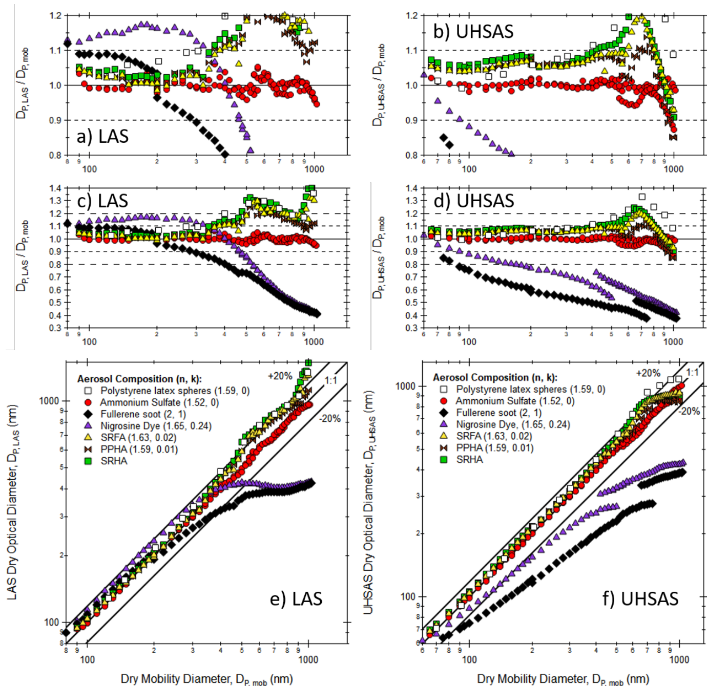
Figure 6: Comparison of optically-sized particle diameter as measured by the LAS (a,c,e) and the UHSAS (b,d,f) to the DMA-classified mobility diameter for the light-absorbing aerosol species listed in Table 1. Both optical sizers were calibrated to ammonium sulphate. The top two rows of panels show the ratio of the optical measurements to the mobility measurements, while the bottommost panels show the data plotted on a 1:1 line ( \pm 20\% indicated). Panels a-d show the same information with panels c and d zoomed in to show additional details. Particles were dried to less than 20% RH with a silica gel diffusion dryer.
