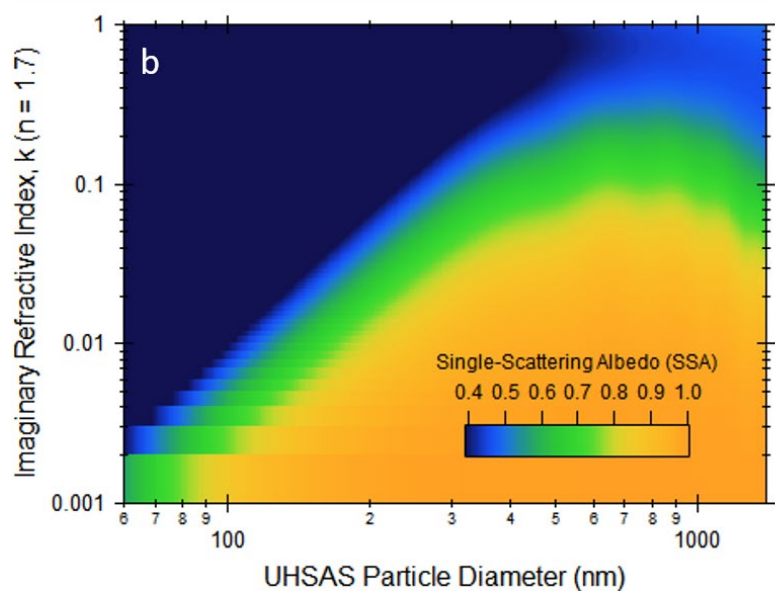
Figure 2: Mie theory calculations of size-resolved particle single-scattering albedo for varying imaginary refractive indices at the LAS laser wavelength of 633 nm (a) and the UHSAS laser wavelength of 1054 nm (b). The real part of the refractive is held constant at 1.7. Unlike Figure 1, these SSA values are computed from the total aerosol scattering and extinction coefficients that are integrated across all angles of the phase function.
