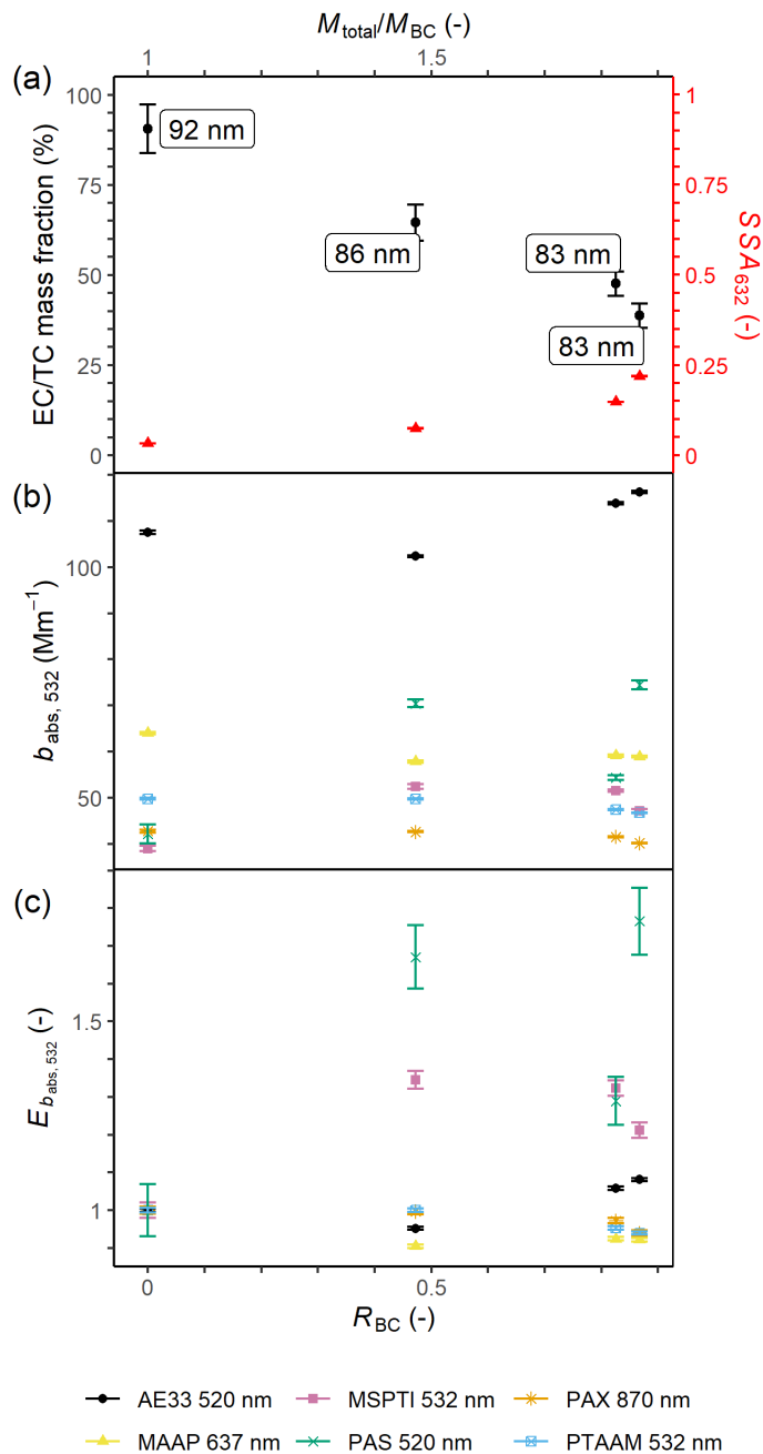
315 | Figure 4: Measurements obtained with Setup 1. (a) EC/TC mass fraction as a function of total mass to BC mass ratio and R_{BC} . The total mass to BC mass ratio and R_{BC} are based on TEOM measurements. The single-scattering albedo (SSA) at 632 nm, calculated from b_{abs} measured by the MAAP and the scattering coefficient measured by the nephelometer, is shown on the secondary y-axis. The sample geometric mean diameter is shown as a label on each data point. (b) Absorption coefficient ( b_{abs} ) as a function of total mass to BC mass ratio and R_{BC} . All b_{abs} values have been converted to a wavelength of 532 nm using the absorption Ångström exponents determined from the fit over all the b_{abs} values from the PTAAM aethalometer. The legend below Figure 4c indicates the wavelengths at which the measurements were performed. All b_{abs} have also been normalized/scaled
