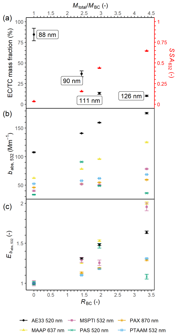
295 Figure 3. Measurements obtained with Setup 0.1. (a) EC/TC mass fraction as a function of total mass to BC mass ratio and R_{BC} . The total mass to BC mass ratio and R_{BC} are based on TEOM measurements. The single-scattering albedo ( SSA ) at 632 70 nm, calculated from b_{abs} measured by the MAAP and the scattering coefficient measured by the nephelometer, is shown on the secondary y-axis. The sample geometric mean diameter is shown as a label on each data point. (b) Absorption coefficient ( b_{abs} ) as a function of total mass to BC mass ratio and R_{BC} . All b_{abs} values have been converted to a wavelength of 532 nm using the absorption Ångström exponents exponents determined from the b_{abs} values from of the PTAAM determined from the fit over all b_{abs} values from the nephelometer. The legend below Figure 3c indicates the wavelengths at which the measurements were
