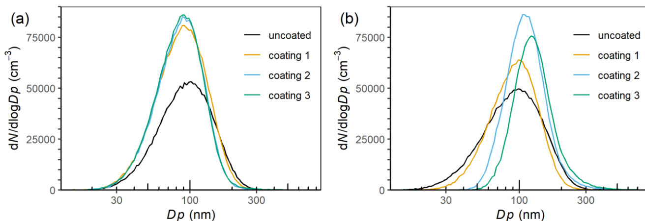
245 Figure 2. Mobility size distributions as measured by SMPS (a) with Setup 1 and (b) with Setup 0.1.
