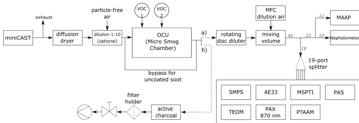
Figure 1. Schematic of experimental setup. The numbers above the arrows indicate aerosol flows in L \text{ min}^{-1} .
