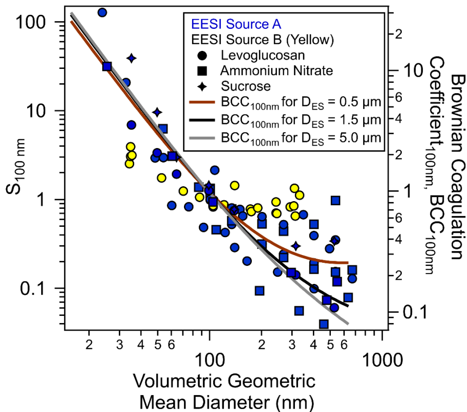
335 Figure 2. Sensitivities of EESI-TOF towards various standards normalized to their respective values at 100 nm as a function of the particle volumetric geometric mean diameter. Blue and yellow markers indicate EESI sources A and B which were initially developed for TOF and Orbitrap mass analyzers, respectively (Lopez-Hilfiker et al., 2019; Lee et al., 2020). Different marker types (●), (■), (◆) denote levoglucosan, \text{NH}_4\text{NO}_3 and sucrose, respectively. The Brownian coagulation coefficients are calculated using the range of ES parent droplet sizes estimated based on our ES operating parameters (Figures S6 and S7). Note: Some of the data points may overlap at the similar volumetric geometric mean diameter due to repetitions of the same experiment settings.
