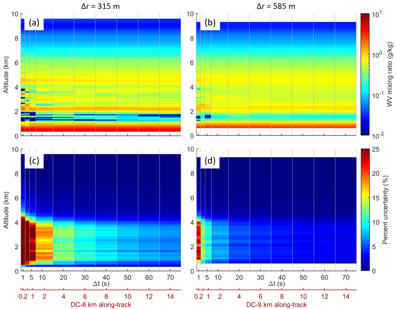
Figure 3. Plots showing (a, b) WV mixing ratio and (c, d) the associated statistical uncertainty for different temporal and range resolutions for a single profile centered at 25.04 UTC from the 2019-04-29 flight (this profile is also shown in Fig. 4). (a, c) have \Delta r = 315 m throughout the profile while (b, d) have \Delta r = 585 m. The x-axis indicates different temporal resolutions ( \Delta t ), which translate to along-track horizontal resolution calculated for the typical DC-8 flight speed.
