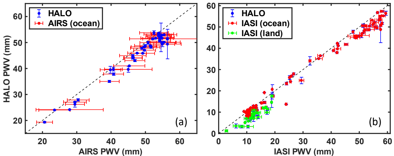
620 Figure 11. Comparison of (a) AIRS or (b) IASI PWV with the average HALO PWV calculated within each satellite retrieval footprint. Bars for AIRS are the reported retrieval uncertainties. Bars for HALO and IASI are standard deviations. Dashed line is 1:1, for reference.
