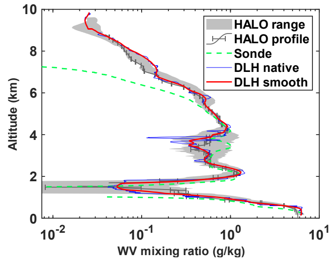
535 Figure 7. HALO comparisons to DLH and sonde from the descent on 04/30. The blue line is the DLH data at native resolution. The red line is DLH smoothed with a 315 m rolling average to match the constant 315 m vertical resolution of the HALO profile. The gray area shows the range of HALO measurements in the area of the spiral descent from the preceding overpass, indicating the expected spatiotemporal variability of the region. An example HALO profile from right before the descent is also shown, with bars denoting measurement statistical uncertainty. The dashed green line shows the malfunctioning sonde profile.
