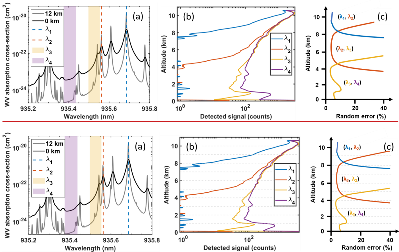
Figure 1. (a) Voigt spectrum of WV absorption cross-section at 12 km (210 hPa, 22K) and at sea level (1013 hPa, 300K), with vertical lines and shading indicating the fixed and tunable HALO wavelengths. (b) Example profile of HALO measured signals for the four transmitted wavelengths, averaged temporally and vertically to match a typical final WV product resolution (60 seconds temporal, 315 m vertical). (c) Sensitivity of line pairs to different parts of the atmosphere, expressed as an estimation of random error versus altitude. Line pairs are in parentheses as (online, offline). Error magnitudes can change with retrieval resolution, as discussed in Section 4.1, though the general line shape versus altitude will remain.
