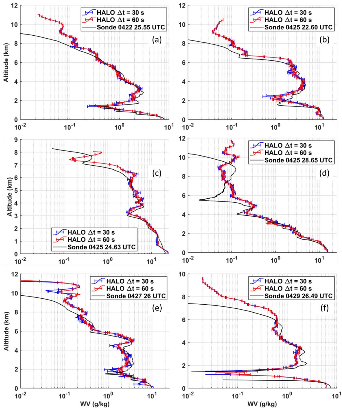
495 Figure 6. HALO WV mixing ratio profiles with statistical uncertainty bars, and collocated dropsonde profiles for comparison. The bars have been decimated for legibility. The sonde WV sensors had erroneous nonlinear damped responses and thus cannot be used for a rigorous quantitative comparison.
