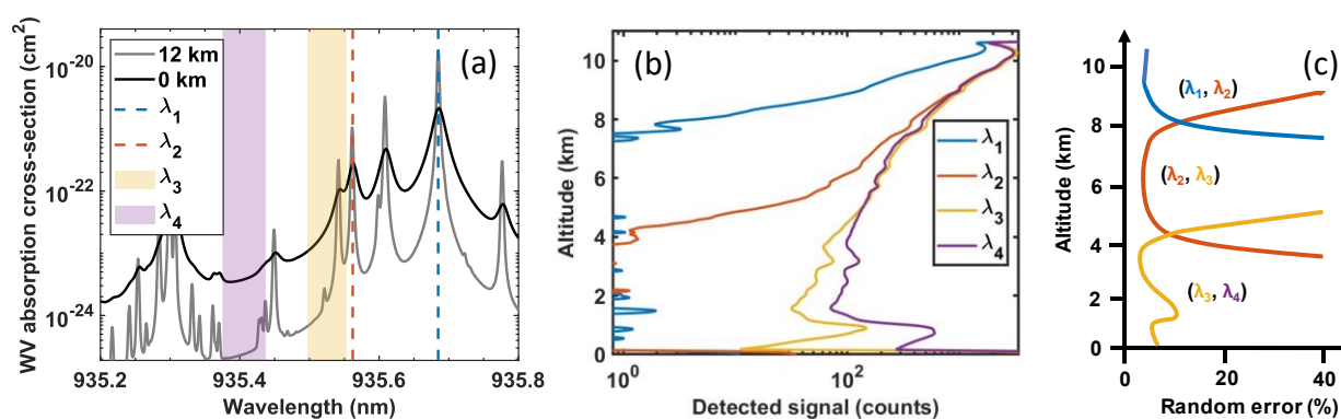
275 Figure 1. (a) Voigt spectrum of WV absorption cross-section at 12 km and at sea level, with vertical lines and shading indicating the fixed and tunable HALO wavelengths. (b) Example profile of HALO measured signals for the four transmitted wavelengths, averaged temporally and vertically to match a typical final WV product resolution (60 seconds temporal, 315 m vertical). (c) 280 Resultant sensitivity of line pairs to different parts of the atmosphere, expressed as an estimation of random error versus altitude. Line pairs are in parentheses as (online, offline).
