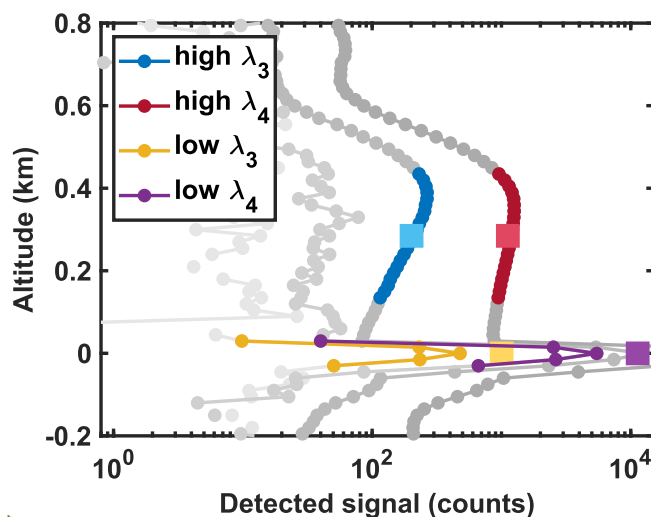
420 Figure 5. Illustration of surface return DIAL concepts. The legend “high” and “low” refer to high gain and low gain channels, plotted at 15 m vertical resolution. The high gain data is temporally averaged to 60 sec, while low gain is a single half second averaged record. The colored circles are averaged (atmospheric) or summed (surface return) to use in the DIAL calculation. These are the P(\lambda, r) inputs to Eq. 1 and are shown as colored squares on the plot. Grayscale points are not used in the surface return but are still shown here for context.
