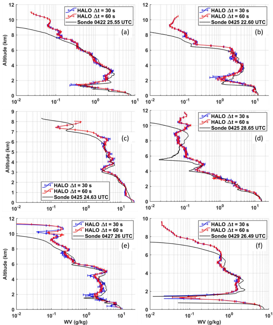
470 Figure 6. HALO WV mixing ratio profiles with statistical uncertainty bars, and collocated dropsonde profiles for comparison. The bars have been decimated for legibility. The sonde WV sensors had erroneous nonlinear damped responses and thus cannot be used for a rigorous quantitative comparison.
