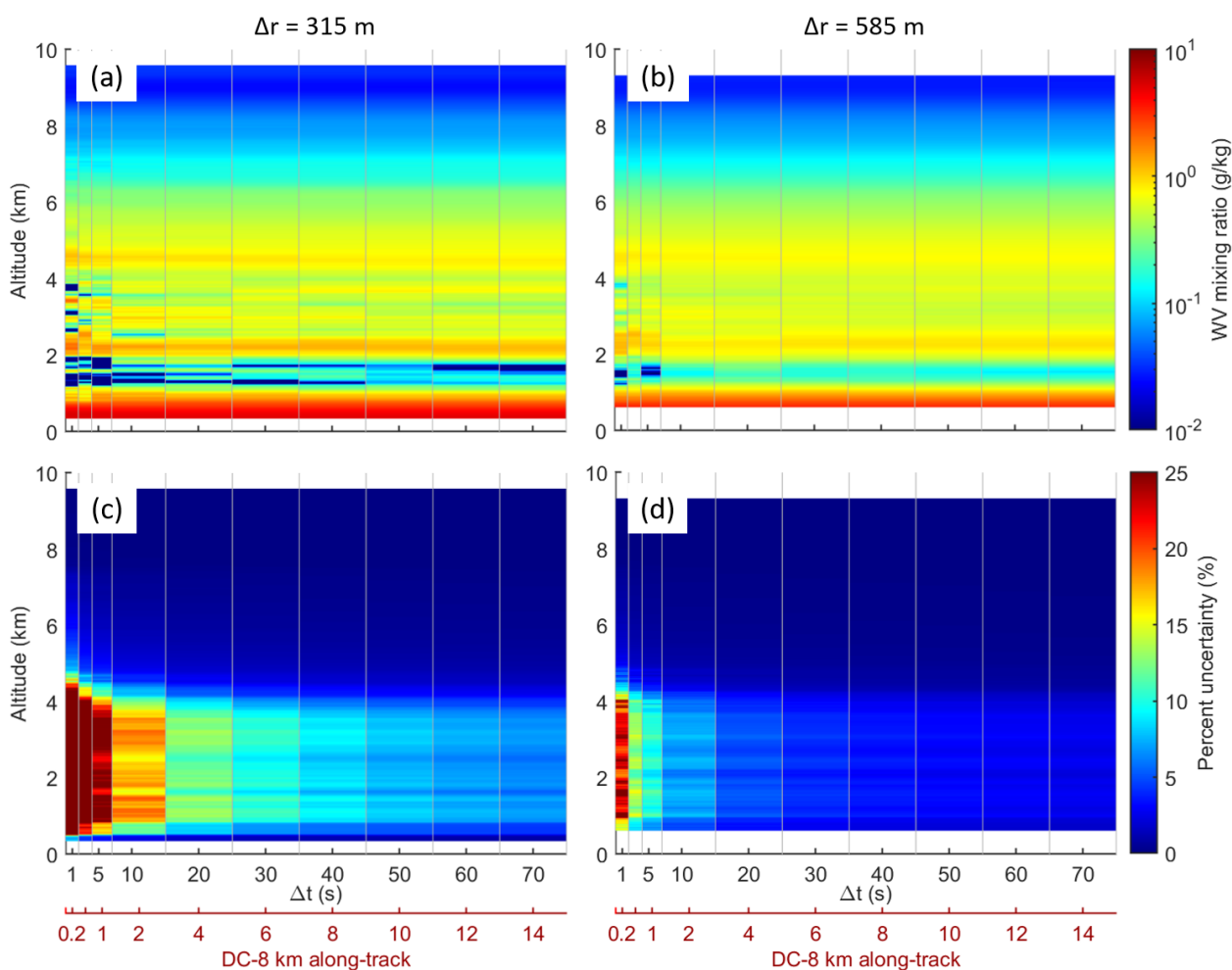
355 Figure 3. Plots showing (a, b) WV mixing ratio and (c, d) the associated statistical uncertainty for different temporal and range resolutions for a single profile centered at 25.04 UTC from the 2019-04-29 flight (this profile is also shown in Fig. 4). (a, c) have \Delta r = 315 m throughout the profile while (b, d) have \Delta r = 585 m. The x-axis indicates different temporal resolutions ( \Delta t ), which translate to along-track horizontal resolution calculated for the typical DC-8 flight speed.
