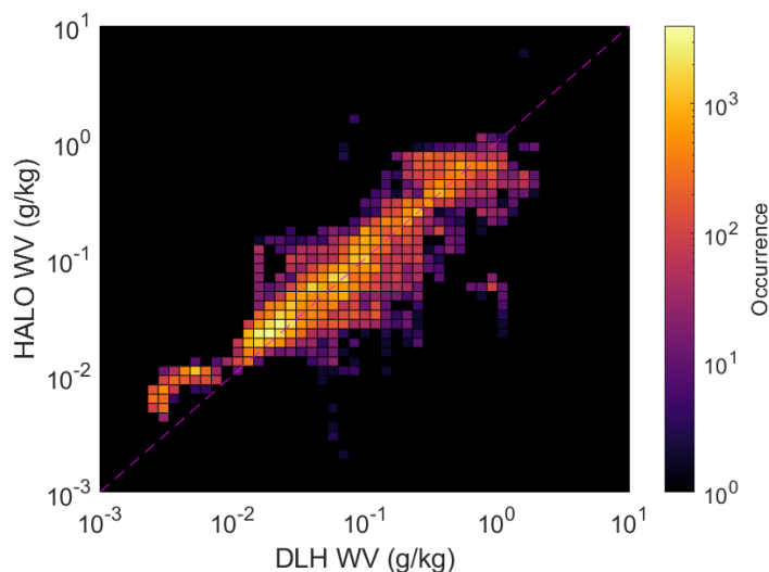
535 Figure 9. Plot of DLH versus HALO WV on log scales and aggregated over all available data, with color indicating the number of points in each bin. The dashed line is a one-to-one line. HALO data is the average of the 5 highest-altitude measurements, ~400 m below the DLH.
