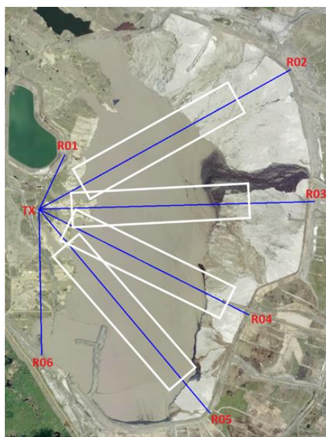
5 Figure 3. Simulated area emission sources (white rectangles) used in SCICHEM modeling scheme for the tailings pond (image credit: CNRL, 2020).
