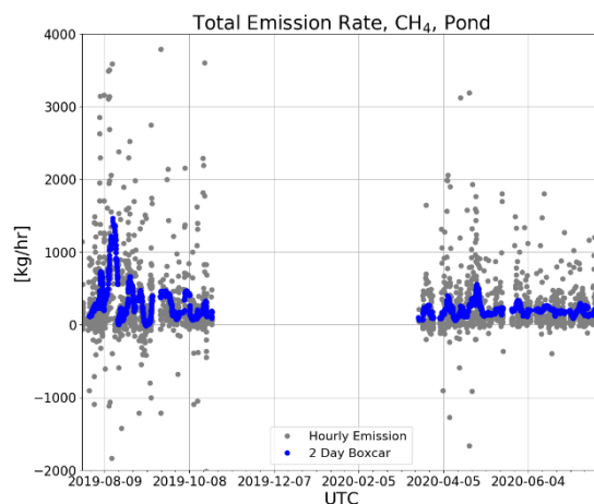
Figure 6. Tailings pond methane emissions.
