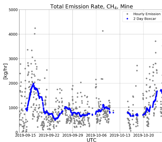
15 Figure 13. Open-pit mine methane emissions.
