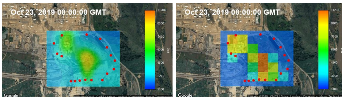
Figure 5. Example plume-based (left) and corresponding box-based (right) methane concentration reconstructions at the open-pit mine.
