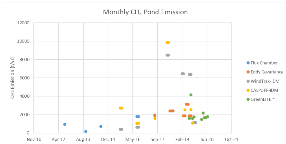
Figure 11. Historical tailings pond emission studies.
