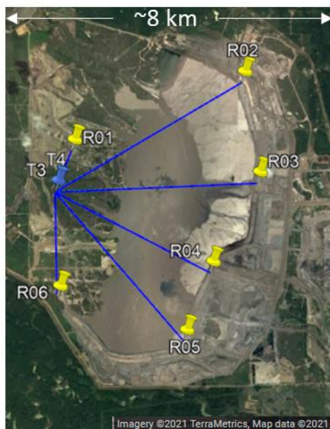
Figure 1. GreenLITE™ system configuration at tailings pond.
