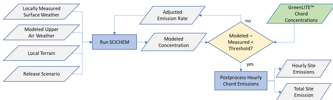
5 Figure 4. Emission estimation flow diagram.
