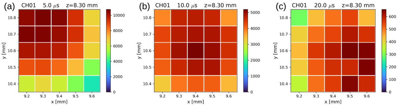
355 Figure 12: Signal mapping (CH01 photon counting signal) of the second session (26 January 2021) at same z and different ranges (a: 5.0 \mu\text{s} - 750 m, b: 10.0 \mu\text{s} - 1500 m, c: 20.0 \mu\text{s} - 3000 m). Here the signal is not normalized due to the lack of sufficient SNR from the second channel in the lower range (highly incomplete overlap).
