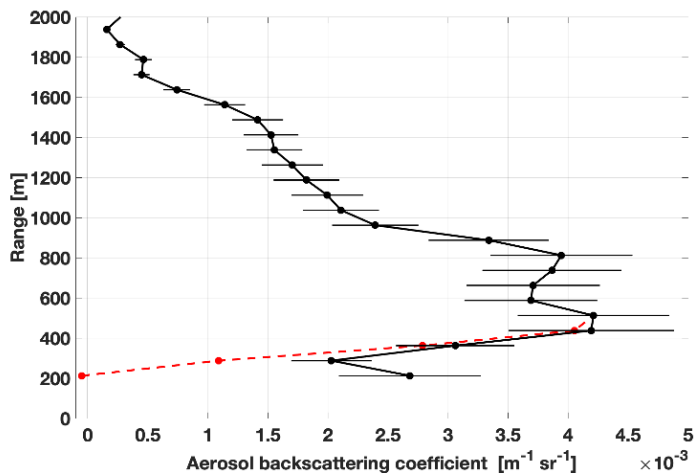
Figure 19: Aerosol backscattering coefficient (11 Feb 2021, 19:45-20:44 UTC), comparison between the overlap-corrected (solid black line) and uncorrected (dashed red line) profile.
