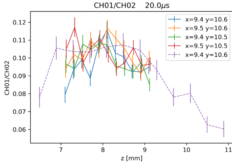
375 Figure 13: Normalized signal at a chosen range (20 \mu s - 3000 m) for different x and y positions as a function of z , data from both mapping sessions (dashed line for the first session, solid line for the second). A plateau is reached approximately between z = 7 mm and z = 9 mm. Each colour corresponds to different x and y positions as indicated in the legend of the plot.
