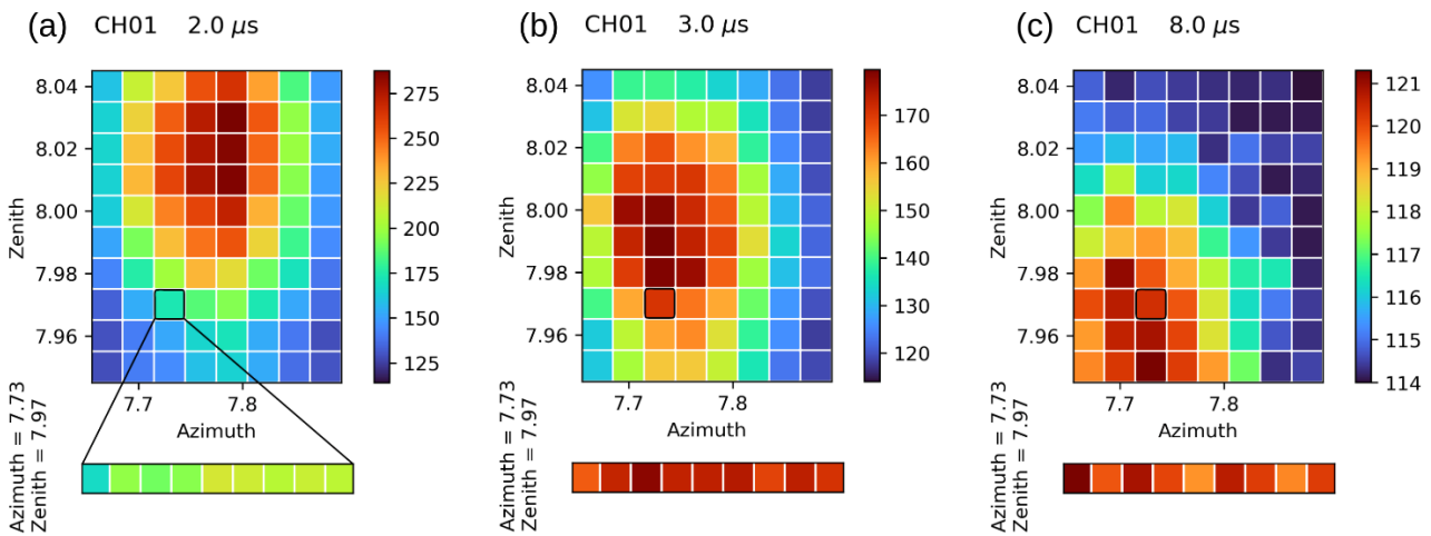
Figure 17: Laser mapping signal (CH01 analogue signal before normalization with the reference position signal) at three different ranges expressed as delays at the top of the bin (a: 2.0 \mu s - 300 m, b: 3.0 \mu s - 450 m, c: 8.0 \mu s - 1200 m). The reference position (Az=7.73 Zen=7.97) is highlighted by the black square. Measurements in this position are acquired every zenith acquisition sequence and are represented in the lower array.
