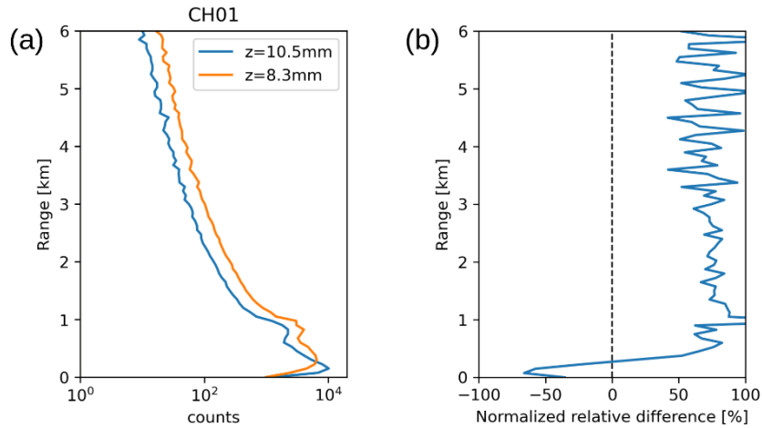
Figure 15: Background subtracted counts (a) and relative difference between the normalized signal CH01/CH02 profiles (b) in the selected position ( x=9.45 mm y=10.55 mm z=8.30 mm) and the starting one ( x=9.40 mm y=10.50 mm z=10.50 mm).
