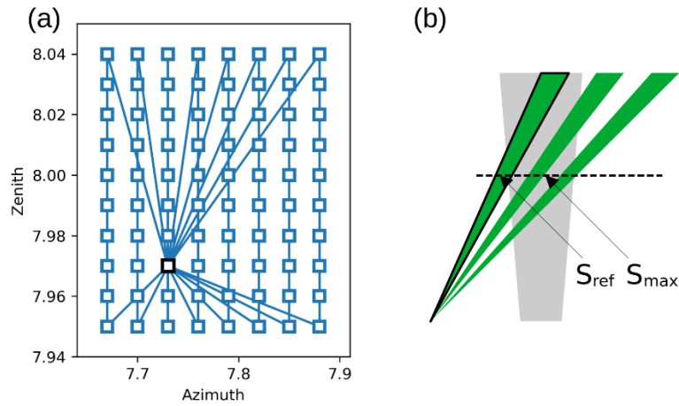
305 Figure 9: (a) Laser mapping scan geometry, after each zenith scan a measurement in the reference position (black square) is 310 performed. (b) Schematic of the telescope FOV and laser beam for different orientations.
