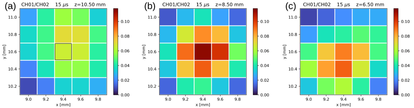
Figure 11: Signal mapping of the first session (13 January 2021) showing the normalized signal for three planes at different z positions and chosen range ( 15 \mu\text{s} - 2250 m AGL). The position derived from the manual alignment is highlighted by the black square.
