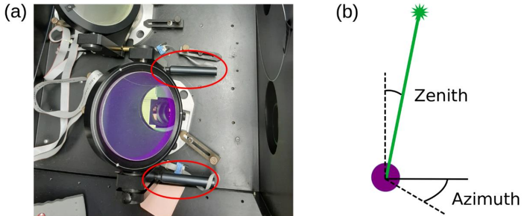
Figure 1: (a) Top view of the two 45° mirrors with azimuth and zenith servomotors (red circled components). (b) Schematic of the mirror/beam movements.
