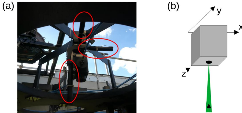
155 Figure 4: (a) Receiving optical system with the 3 axis servomotors (red circled components). (b) Schematic of the receiving block movements.
