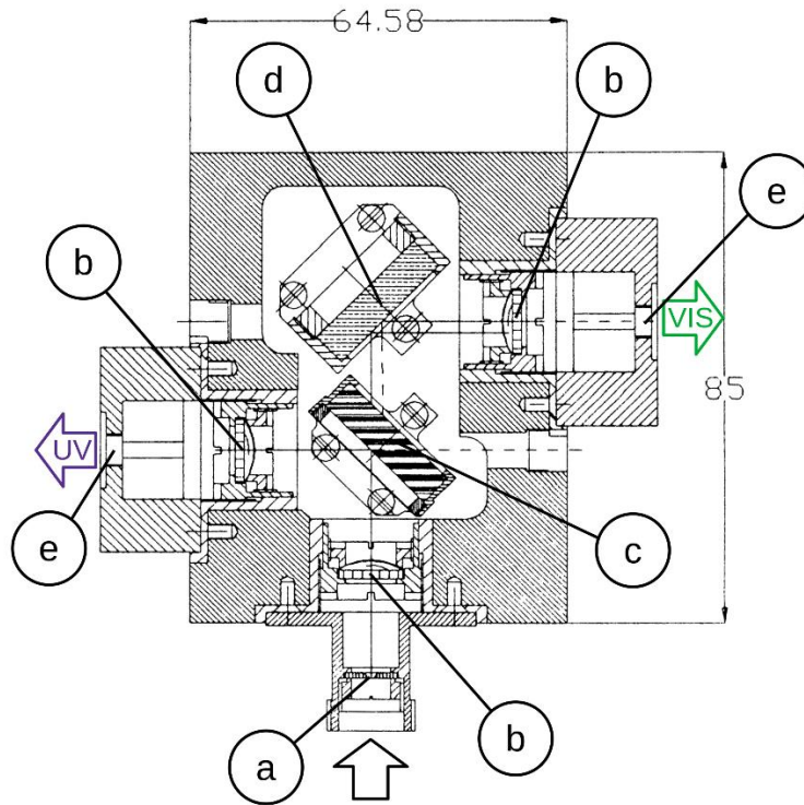
125 Figure 3: Schematics of the receiving block, a: field stop diaphragm (0.8 mm diameter), b: collimation lenses ( f = 20 mm), c: dichroic beam splitter ( \lambda = 440 nm), d: 45^\circ mirror, e: optical fibre connector. Dichroic beam splitter and UV collimation lens are currently not present in the receiving block of the 15 cm telescope.
