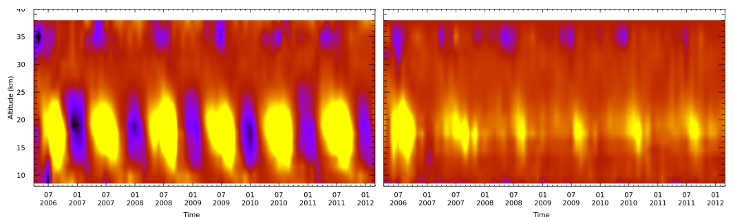
Figure 6. Time series of monthly average CFC-11 ascending-descending difference profiles for V7 (left) and V8 (right) MIPAS/ESA products. The maps refer to the latitude band from 45S to 60S.
