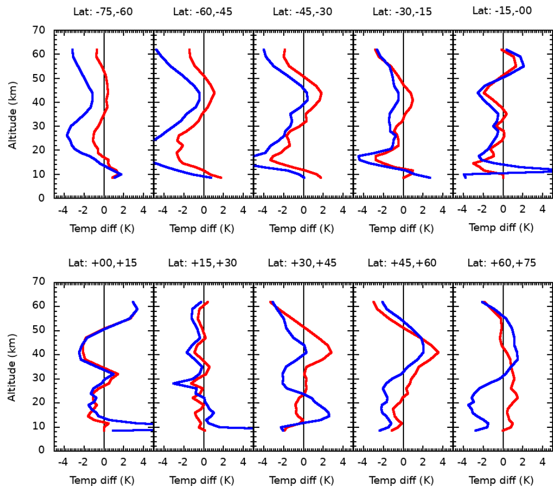
Figure 3. Temperature ascending-descending average difference profiles for V7 (blue) and V8 (red) MIPAS/ESA products. Averaging extends to the measurements acquired in the month of December of the years from 2006 to 2011 (OR part of the mission). The different panels refer to different latitude bands as indicated on the top of the panels.
