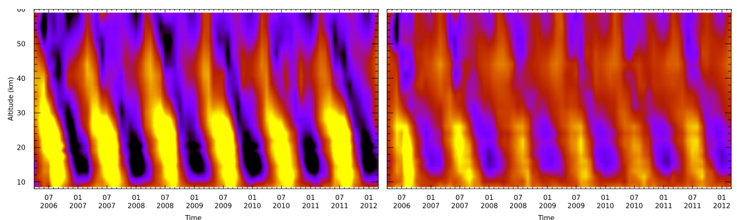
Figure 5. Time series of monthly average temperature ascending-descending difference profiles for V7 (left) and V8 (right) MIPAS/ESA products. The maps refer to the latitude band from 45S to 60S.
