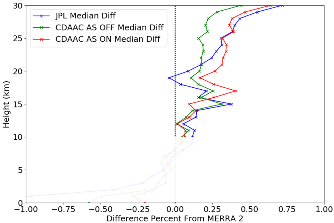
740 Figure 5. Percentage refractivity median differences of the JPL and CDAAC data sets minus the MERRA-2 reanalysis, interpolated to a common 1-km altitude grid. Altitudes between 10 and 30 km are analyzed. Percent difference is with respect to the mean MERRA-2 refractivity at the corresponding altitude.
