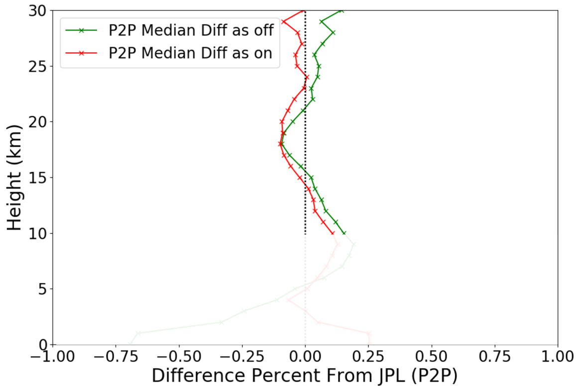
735 Figure 4. Percentage refractivity median difference of JPL minus UCAR AS-on and AS-off for profiles common to the single frequency and UCAR data sets (“P2P” data set). The focus altitudes are 10 km-30 km. Profiles are interpolated to a common 1-km vertical grid spacing. Percent difference is with respect to the mean refractivity at the corresponding altitude.
