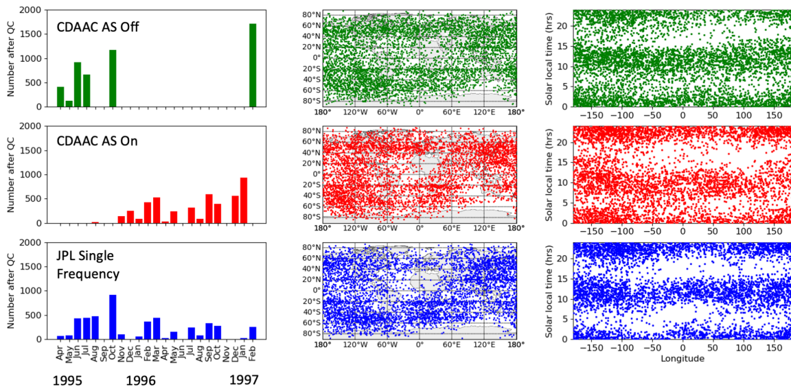
715 Figure 1. Information on the three data sets analyzed: UCAR's CDAAC AS-off, AS-on and JPL single frequency. The left column shows the number of profiles by month, after quality control is applied. The middle column shows the locations of the profiles. The right column shows the solar local time of the profiles versus longitude.
