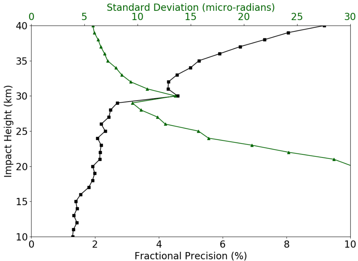
815 Figure 8. Estimates of the standard deviation of the differences (green curve) between single- and dual-frequency bending angle for AS-off conditions using the JPL radio occultation processing chain, for approximately 2000 profiles. The black curve is the precision divided by the mean refractivity at the corresponding altitude. Precision is estimated using the robust statistic of interquartile range divided by 1.349, which corresponds to 1\sigma .
