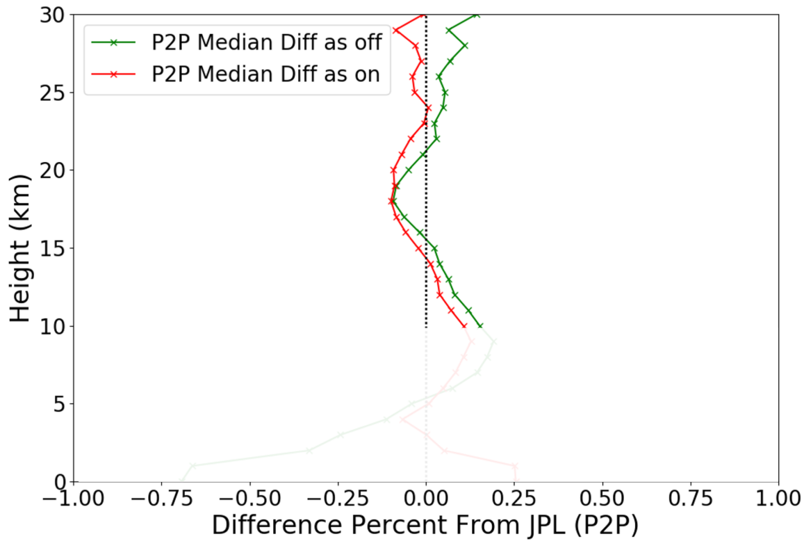
785 Figure 4. Percentage refractivity median difference of JPL minus UCAR AS-on and AS-off for profiles common to the single frequency and UCAR data sets (“P2P” data set). The focus altitudes are 10 km-30 km. Profiles are interpolated to a common 1-km vertical grid spacing. Percent difference is with respect to the mean refractivity at the corresponding altitude.
