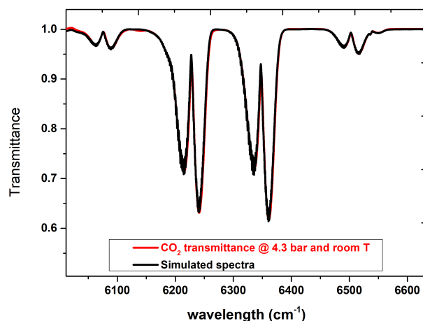
Figure 9. Comparison between acquired \text{CO}_2 spectra @ room temperature and 4.3 bar (red curve) and simulated (black curve)
