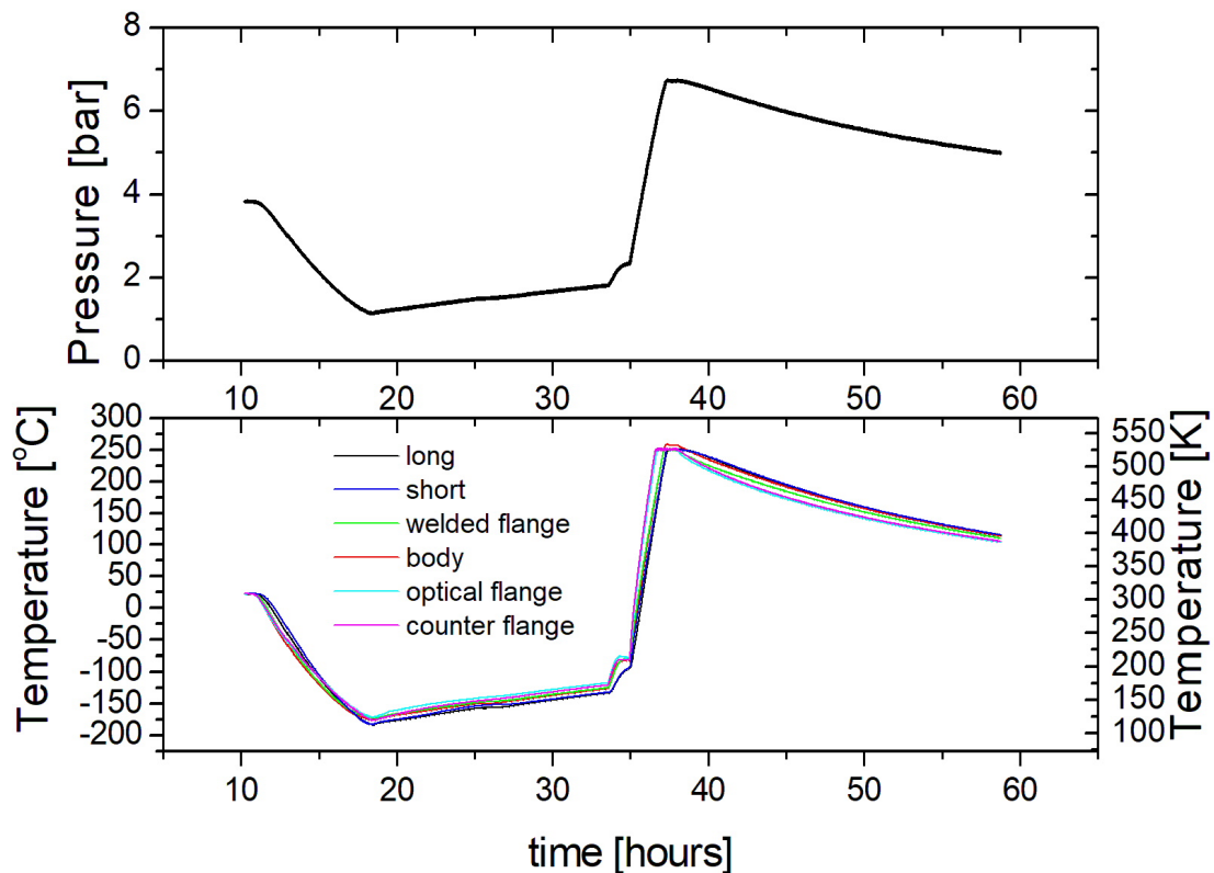
Figure 6. Cooling and heating test of PASSxS with about 3.7 bar of argon in the sample chamber at room temperature. Upper panel: The pressure of the Ar is indicated in bars. Lower panel: The blue and black curves refer to the temperatures recorded by the short and long thermocouples put inside the inner cell (6 and 5 in Figure 2). The light blue, green, violet and purple curves refer to the temperatures acquired by the other thermocouples (4,3,2,1 in Figure 2) .
