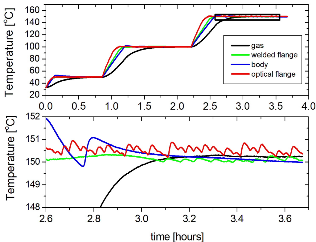
Figure 8. Upper panel: heating and temperature stabilization in three steps. Lower panel (enlarged part of the upper panel, indicated as a black box in the upper panel) : Temperature stability of the different parts of the cell and the gas during active stabilization.
