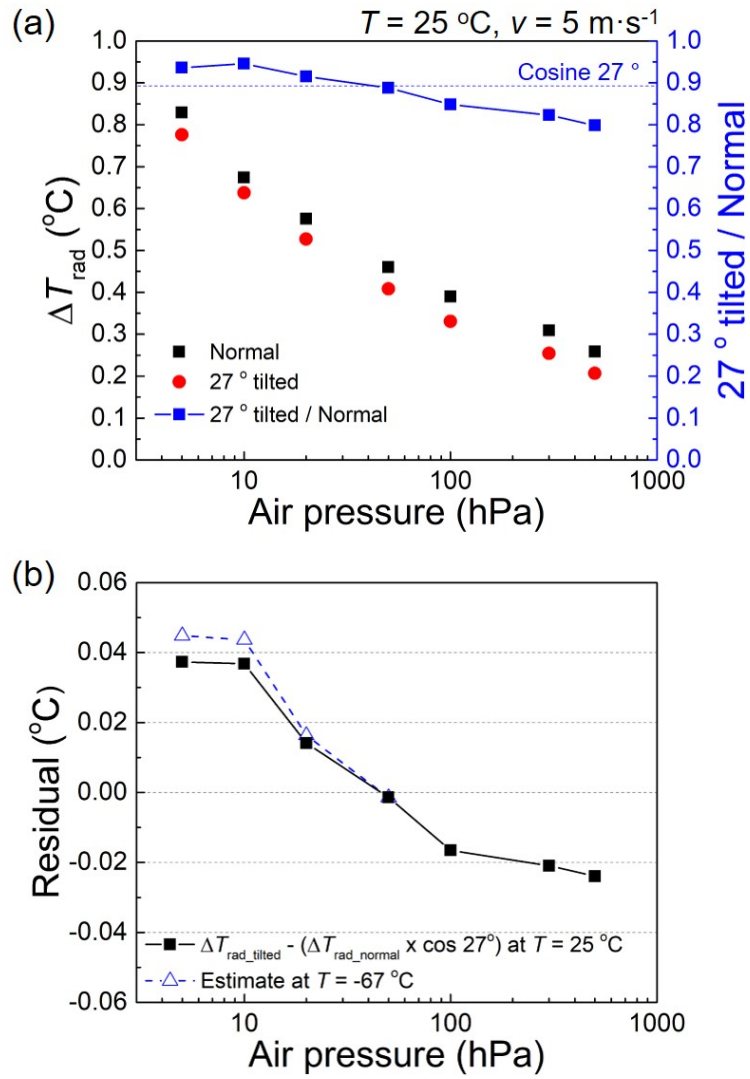
Figure 7. (a) Effect of tilting of the sensor boom showing (left y-axis) \Delta T_{\text{rad}} with normal ( \Delta T_{\text{rad\_normal}} ) and 27° tilted position ( \Delta T_{\text{rad\_tilted}} ) and the ratio between them (right y-axis). (b) Residual between \Delta T_{\text{rad\_tilted}} and \Delta T_{\text{rad\_normal}} \times \cos 27^\circ at T = 25 \text{ }^\circ\text{C} and the estimate of the residual at T = -67 \text{ }^\circ\text{C} by using Eqs. (6), (7), and (8).
